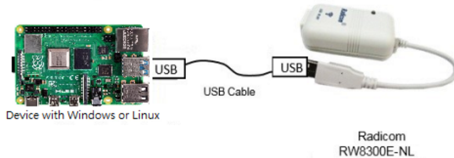
Environment of RW8300E-NL updating firmware
