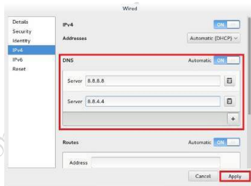
After set DNS
