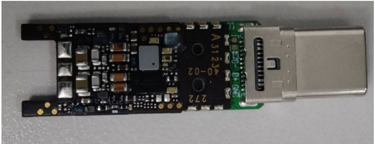
Bottom photo of PCB
