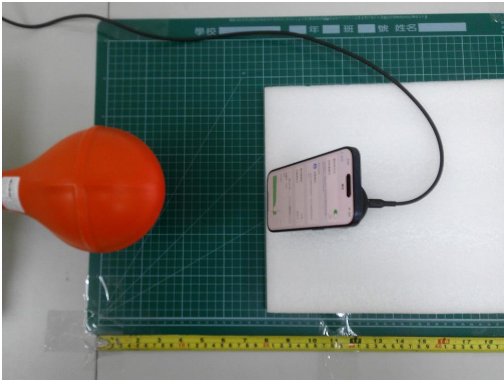
E-Field and H-Field (Z-axis Above)
