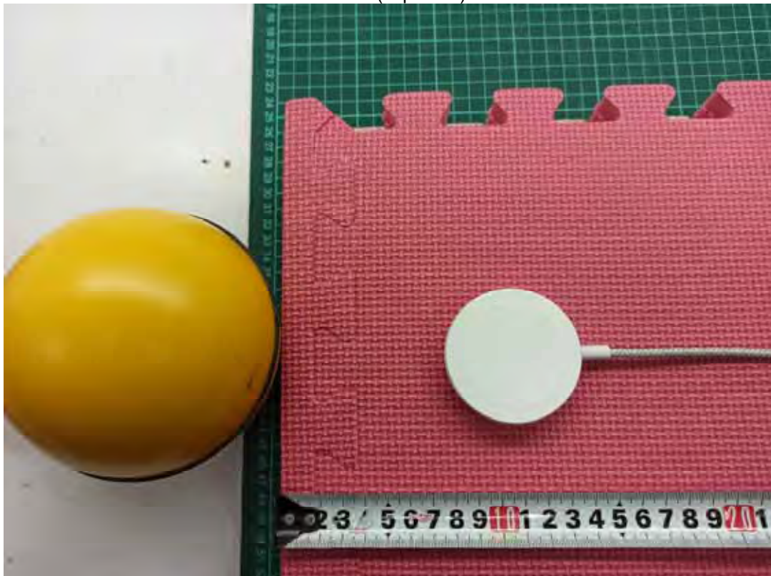
H-Field (Bottom: 8cm)
