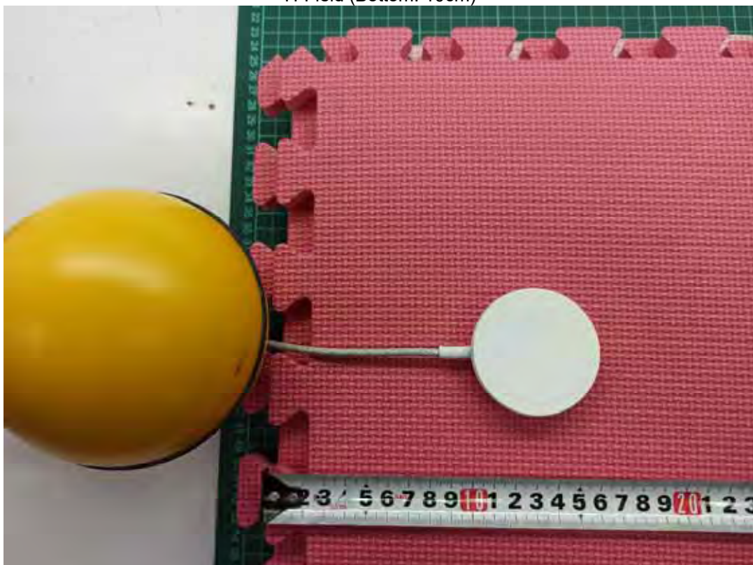
H-Field (Bottom: 10cm)
