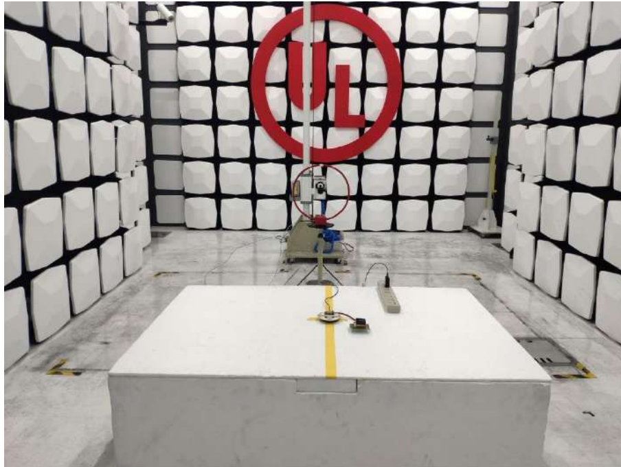
10W load
