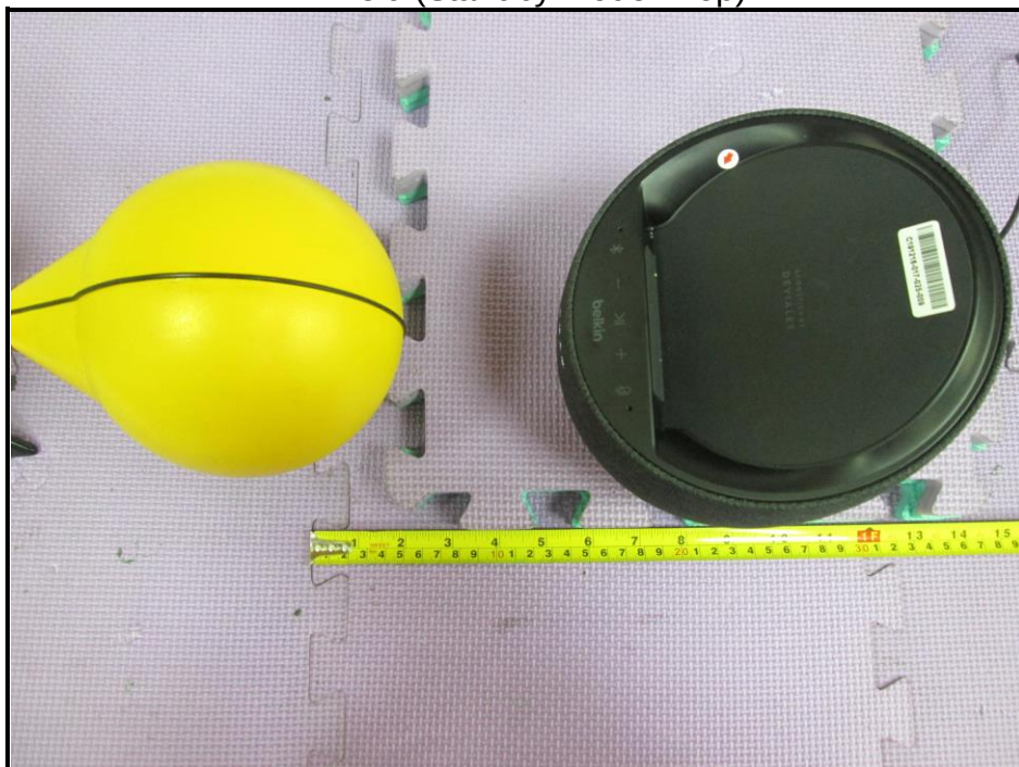
H-Field (Standby Mode - Top)
