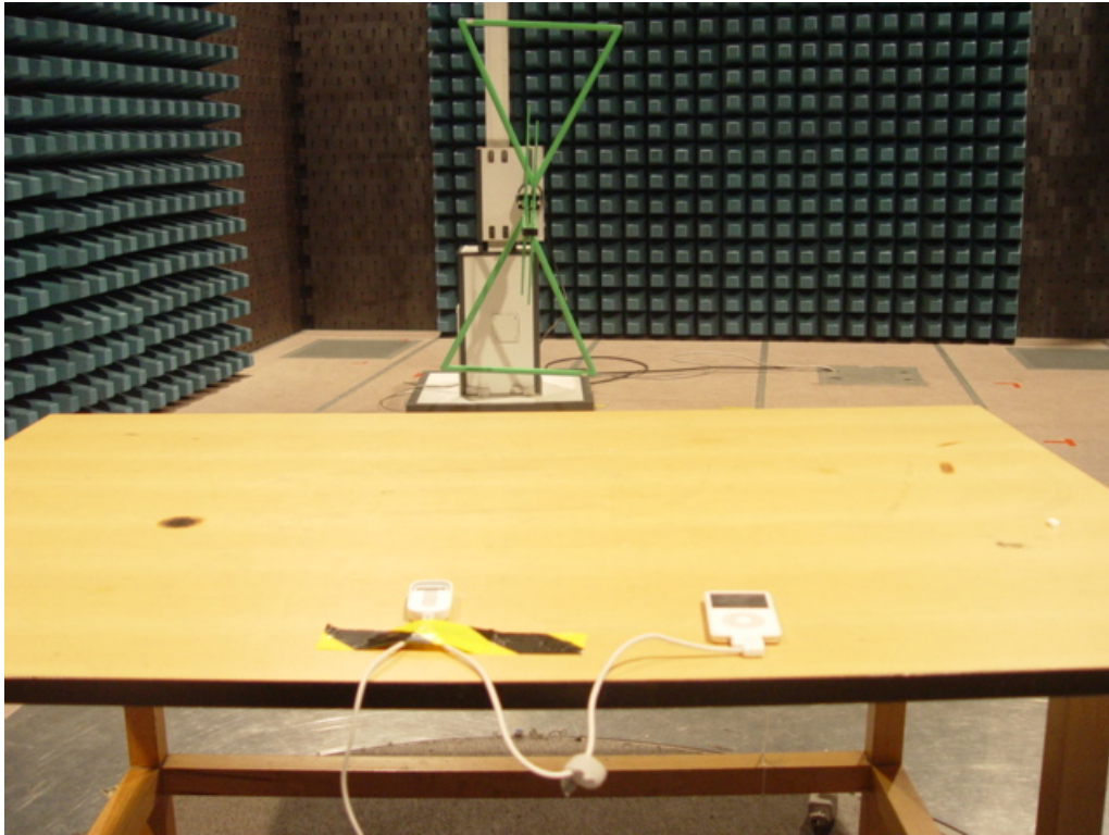
Photo 1: Radiated test photo
