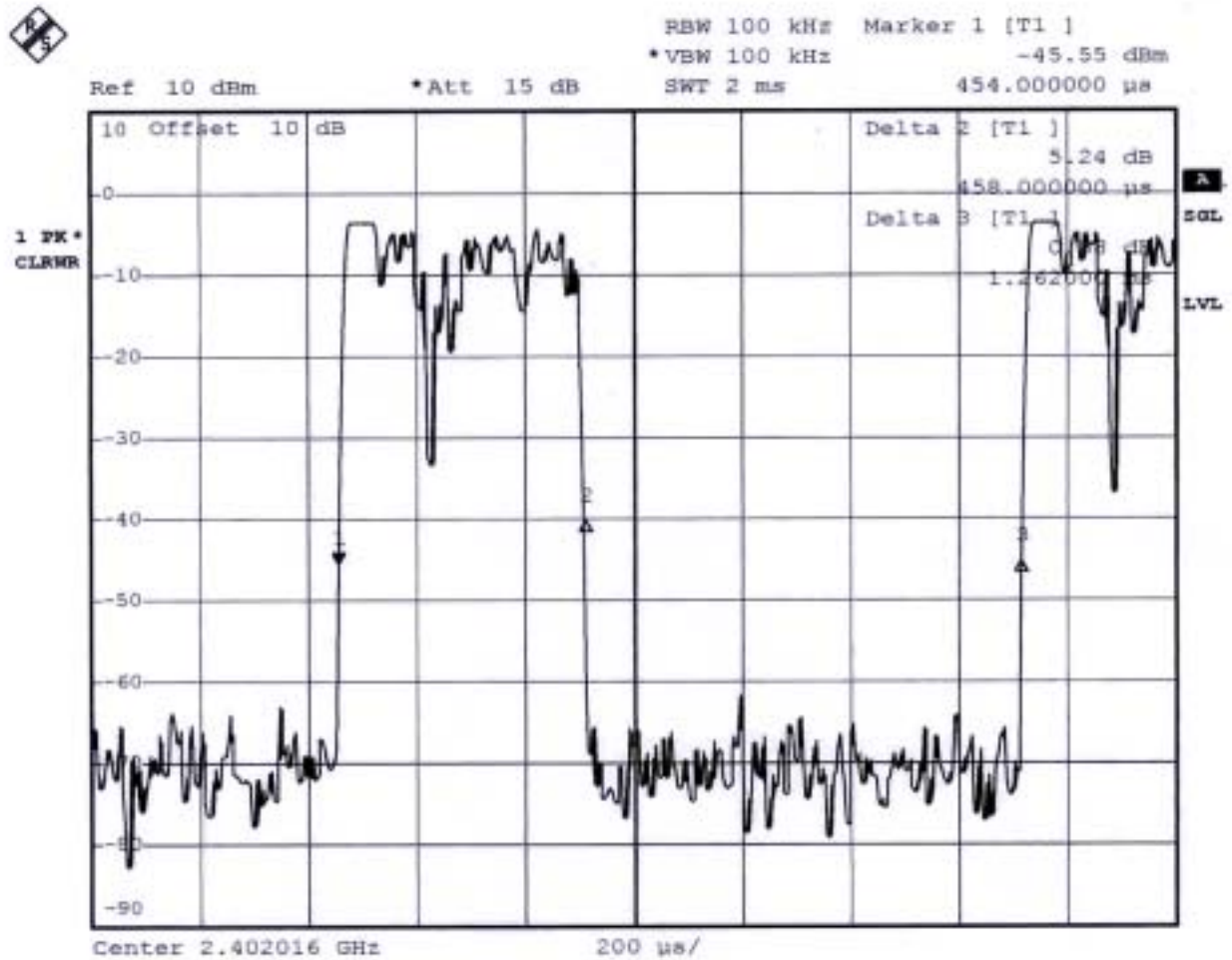
Plot 1 (Channel 00)
