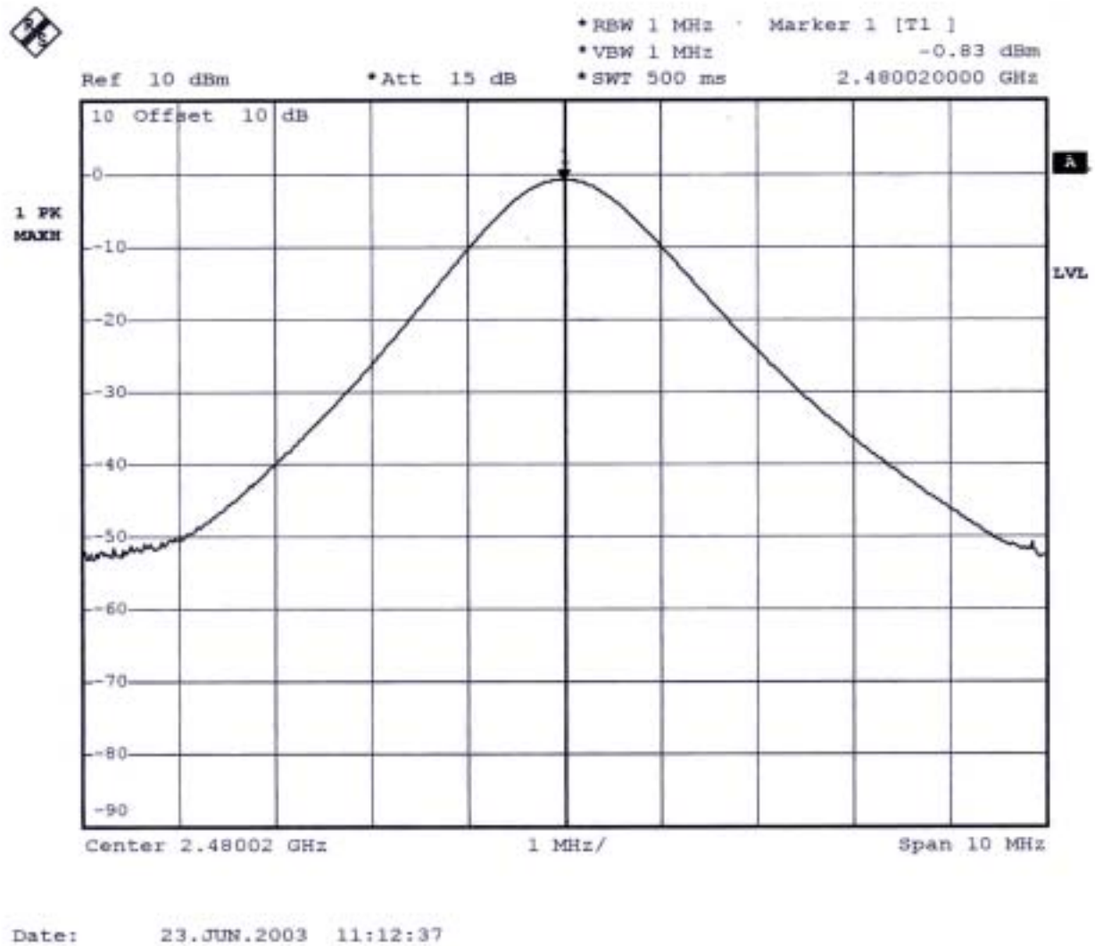
Plot 3 (Channel 78)
