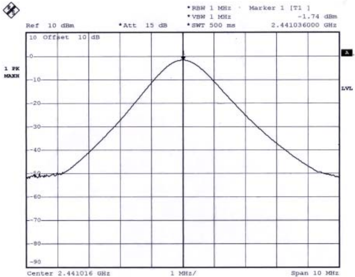
Plot 2 (Channel 39)
