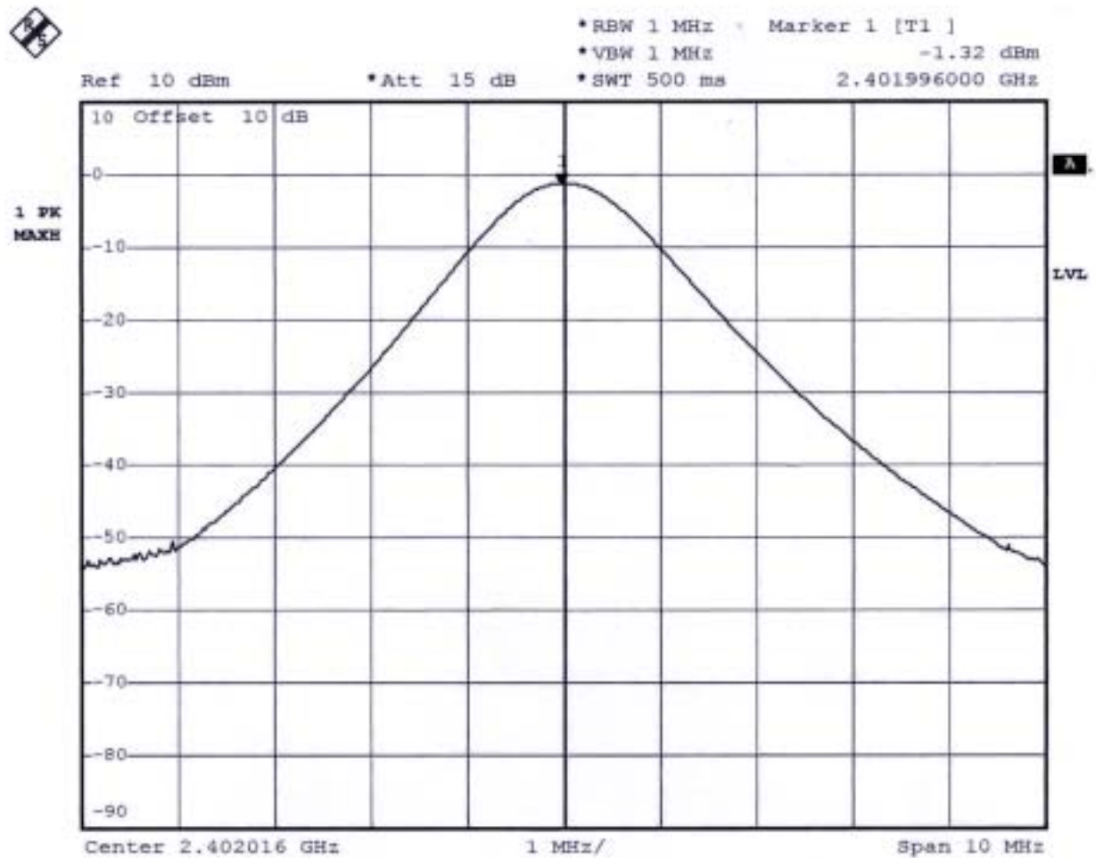
Plot 1 (Channel 00)
