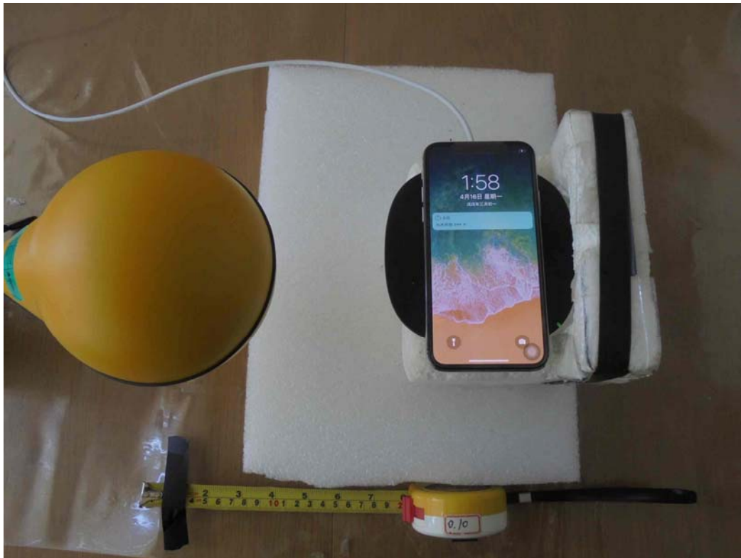
H-Field (Charging Mode with iPhone X - Left)
