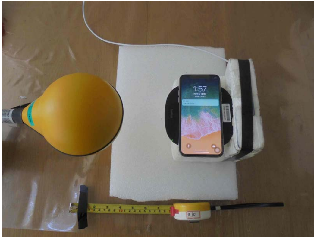
H-Field (Charging Mode with iPhone X - Top)
