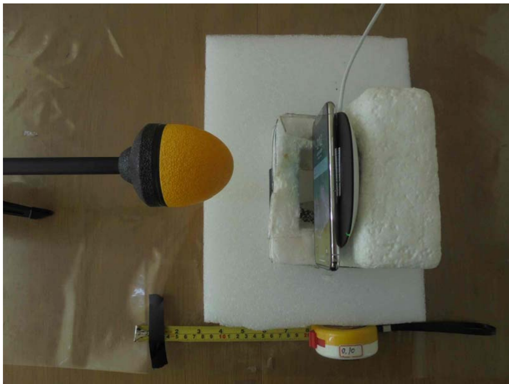
E-Field (Charging Mode with iPhone X - Z-axis)
