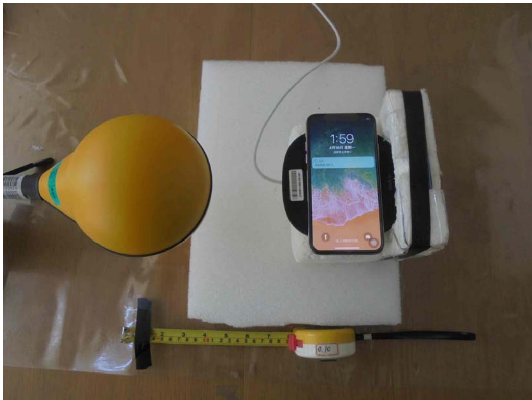
H-Field (Charging Mode with iPhone X - Bottom)
