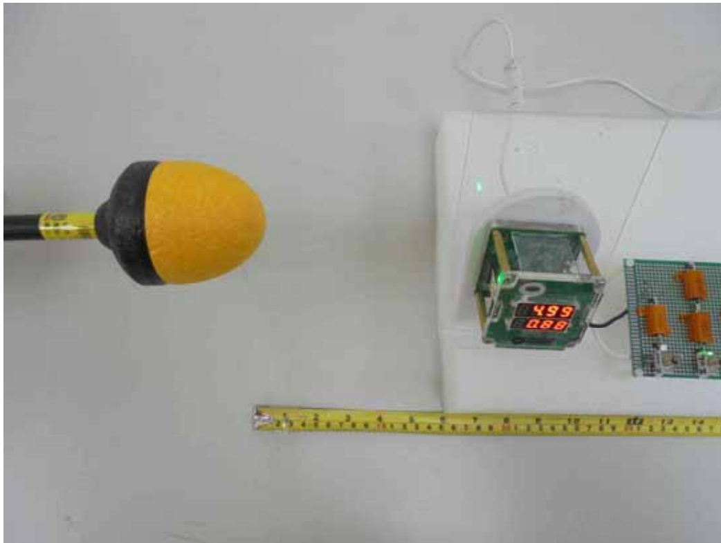
E-Field (Charging Mode with Load with 3mm airgap - Left)
