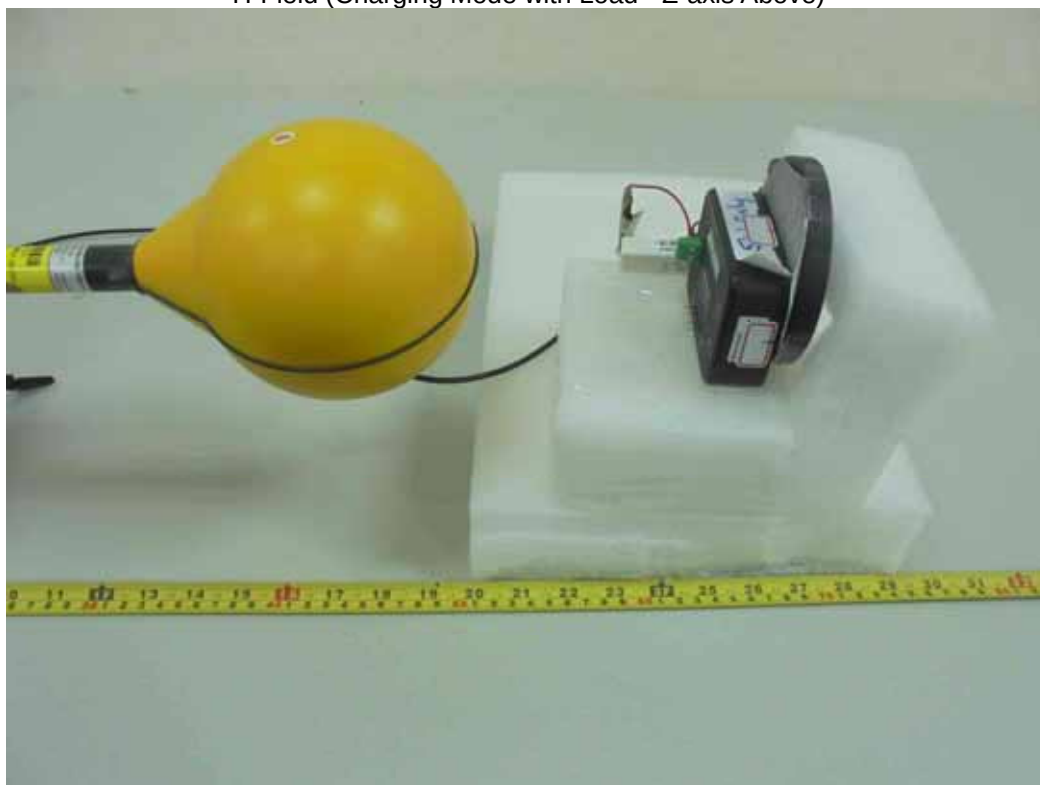
H-Field (Charging Mode with Load - Z-axis Above)
