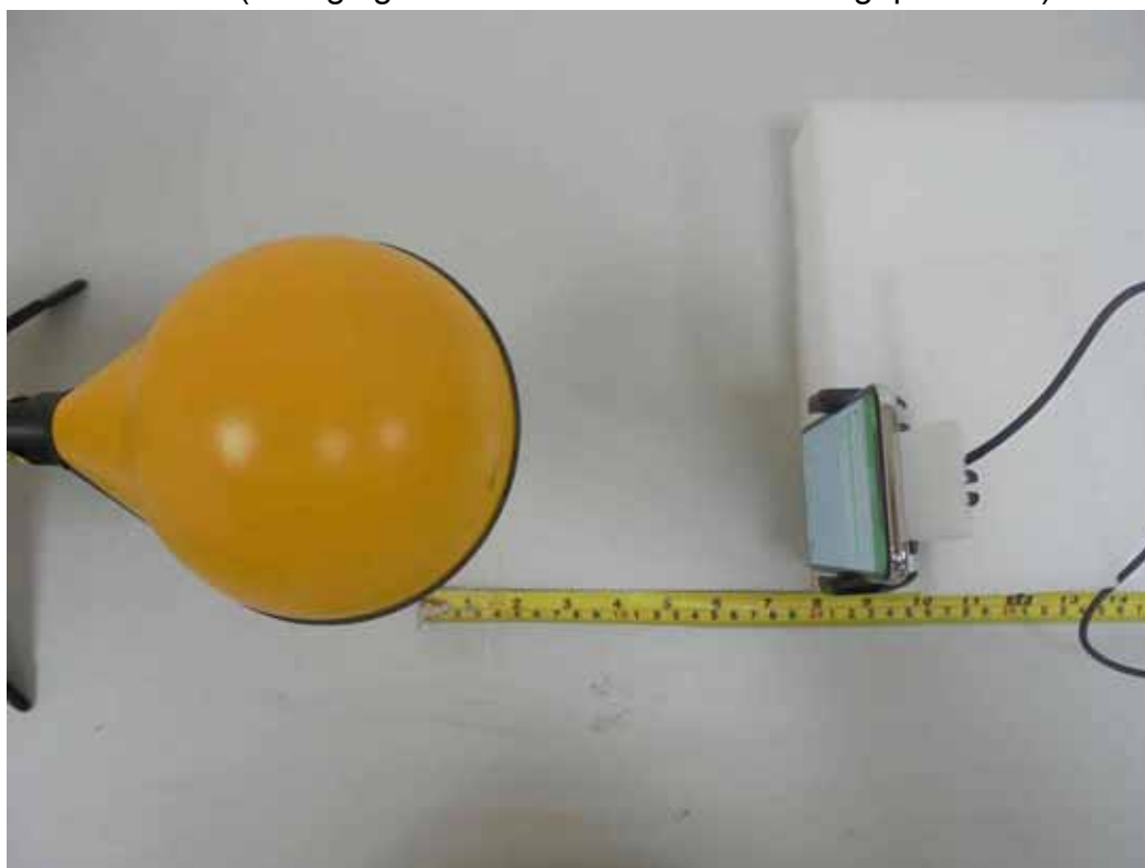
H-Field (Charging Mode with iPhone with 3mm gap - Z-axis)
