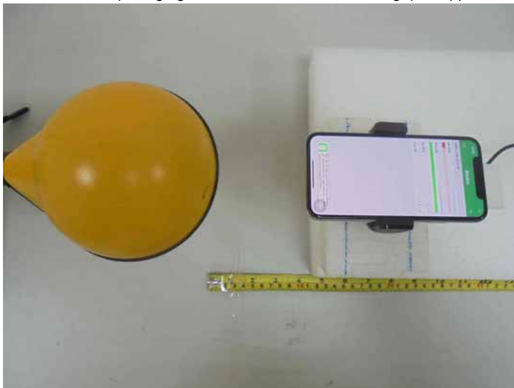
H-Field (Charging Mode with iPhone with 3mm gap - Top)
