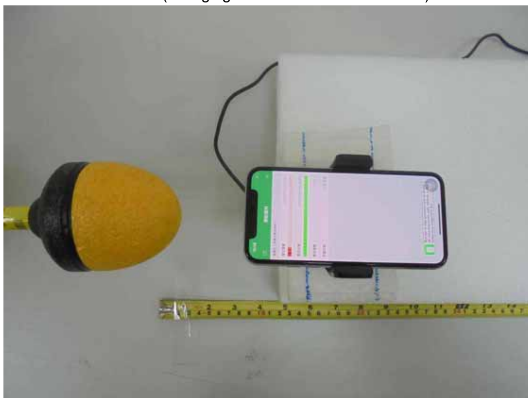
E-Field (Charging Mode with iPhone - Bottom)
