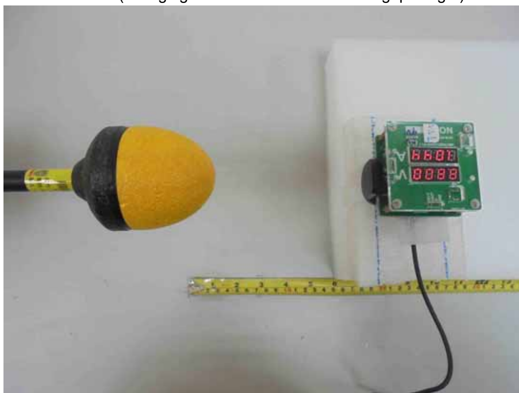
E-Field (Charging Mode with Load with 3mm gap - Right)
