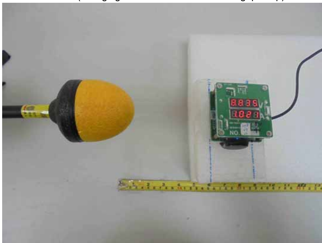
E-Field (Charging Mode with Load with 3mm gap - Top)
