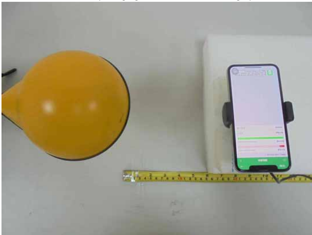
H-Field (Charging Mode with iPhone - Right)
