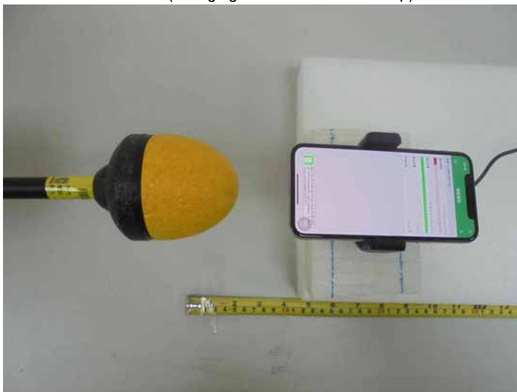
E-Field (Charging Mode with iPhone - Top)
