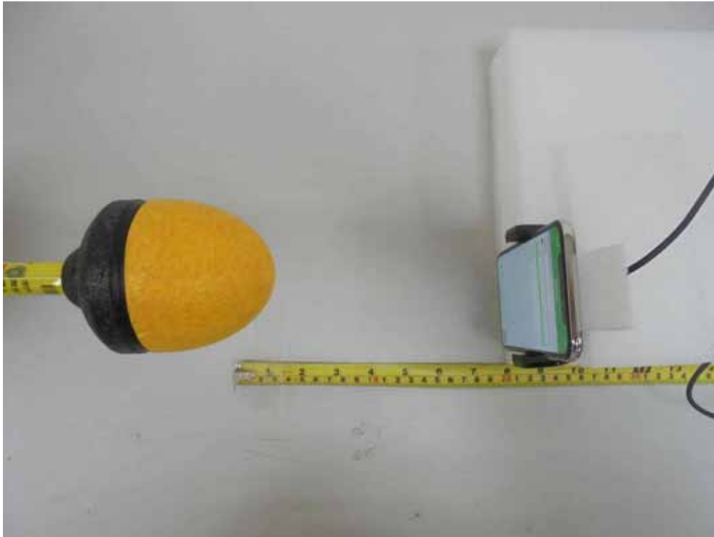
E-Field (Charging Mode with iPhone with 3mm gap - Z-axis)
