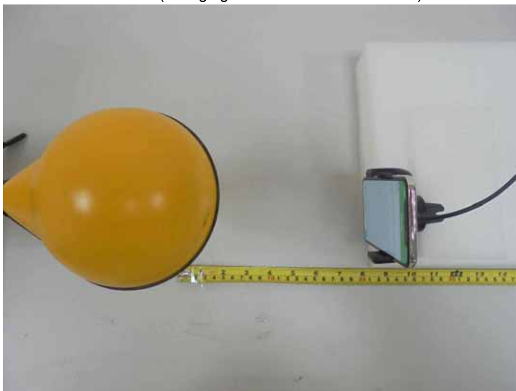
H-Field (Charging Mode with iPhone - Z-axis)
