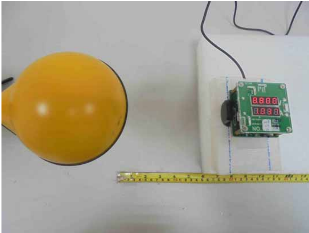
H-Field (Charging Mode with Load with 3mm gap - Left)
