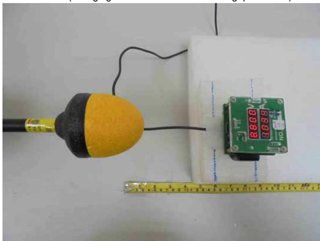
E-Field (Charging Mode with Load with 3mm gap - Bottom)
