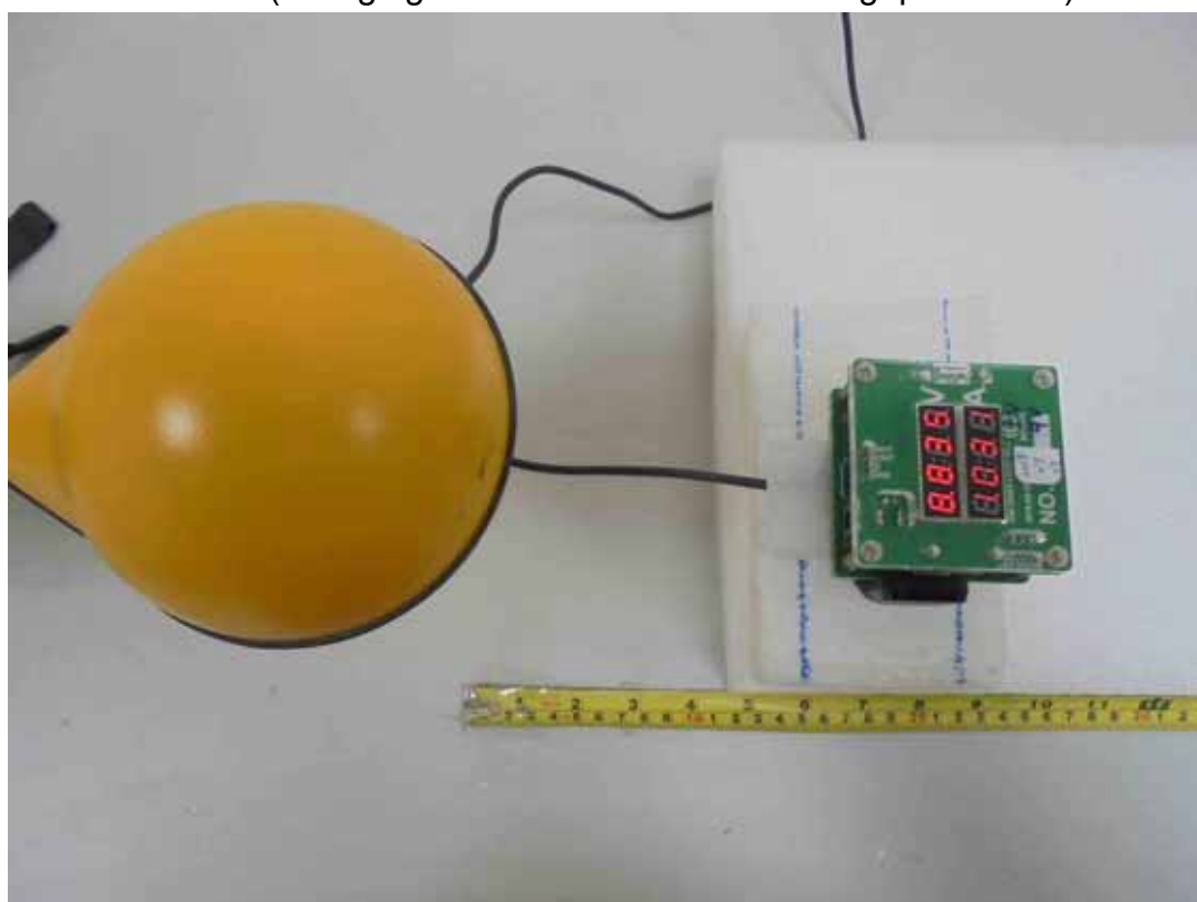
H-Field (Charging Mode with Load with 3mm gap - Bottom)
