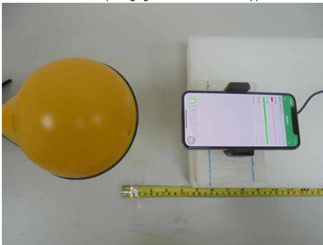
H-Field (Charging Mode with iPhone - Top)
