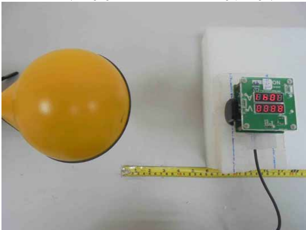
H-Field (Charging Mode with Load with 3mm gap - Right)
