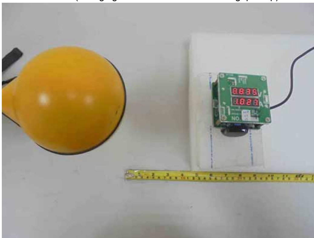
H-Field (Charging Mode with Load with 3mm gap - Top)
