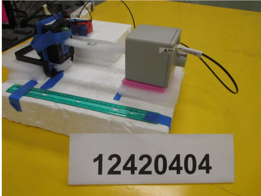
CENTER, RF EXPOSURE SETUP PHOTO
