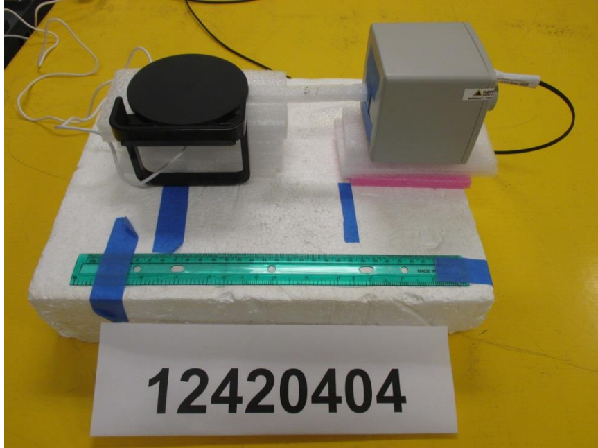
S4, RF EXPOSURE SETUP PHOTO
