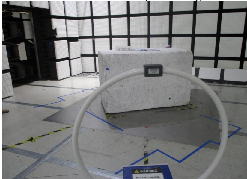
RADIATED EMISSIONS BELOW 30MHz (Back- Standby)
