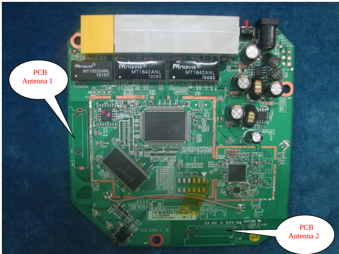
PCB Antenna
