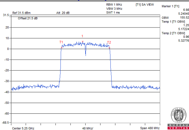
802.11ax (HE160)_Chain 0 / 50
