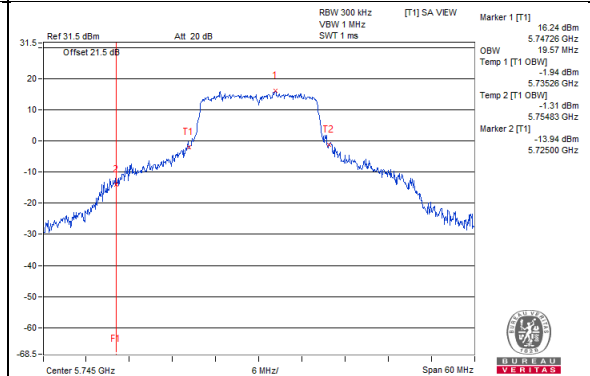
802.11a_Chain 3 / CH149
