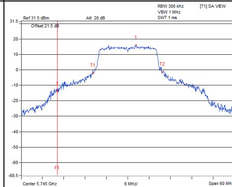
802.11a_Chain 3 / CH149
