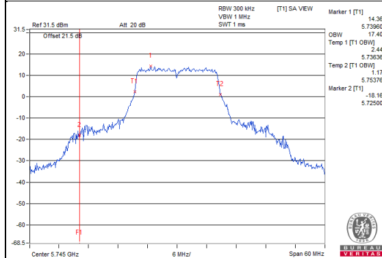
802.11a_Chain 2 / CH149
