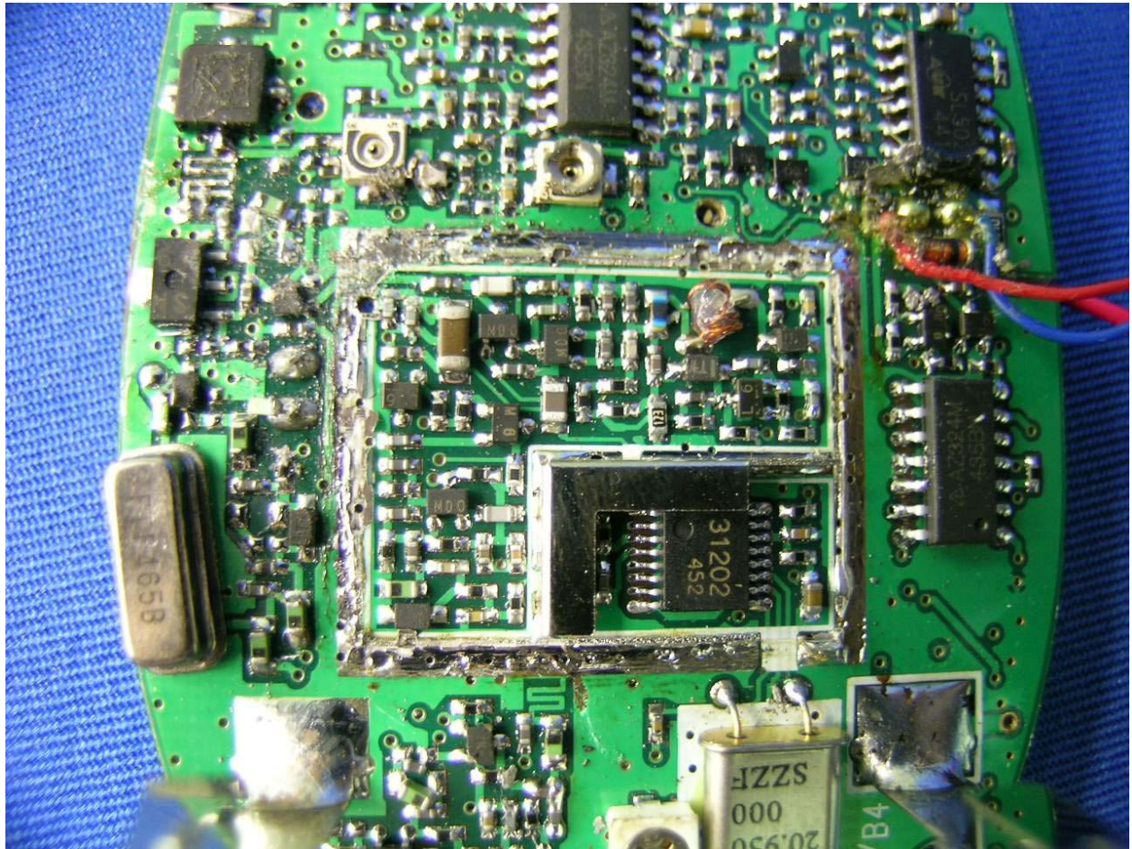
Internal Photo -4
