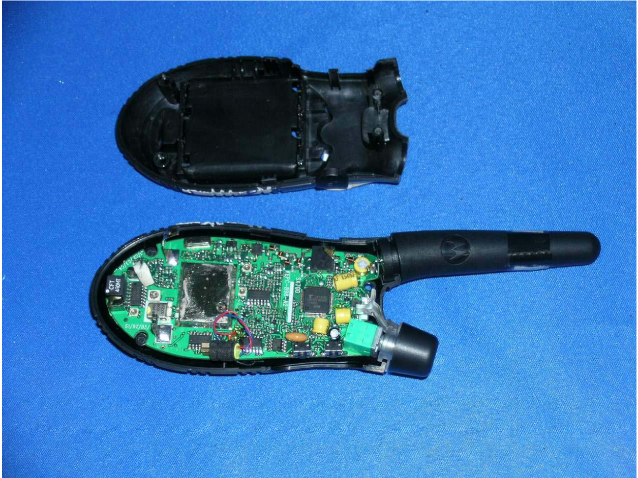
Internal Photo - 1
