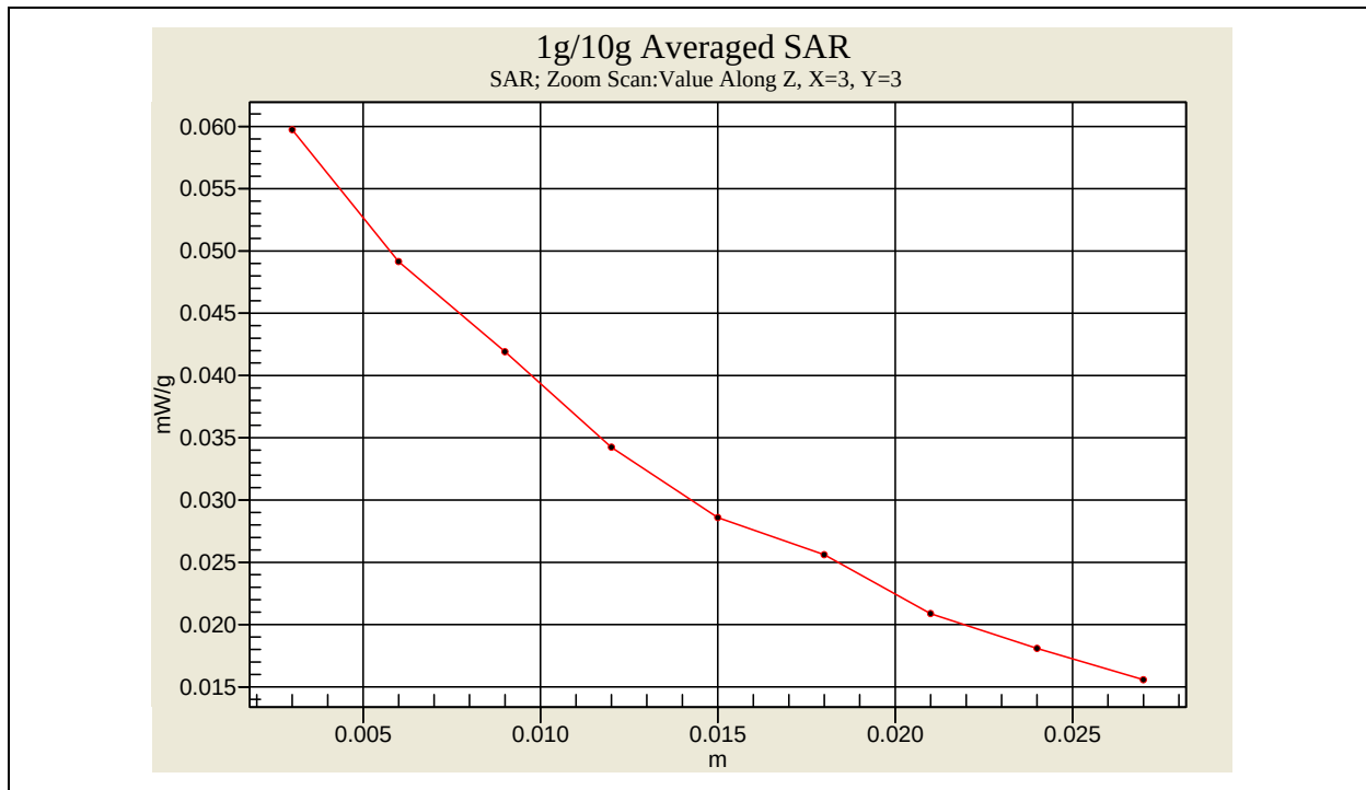
FRS Body SAR - 15 mm Spacing _ CH11 (Ni-MH Battery)
