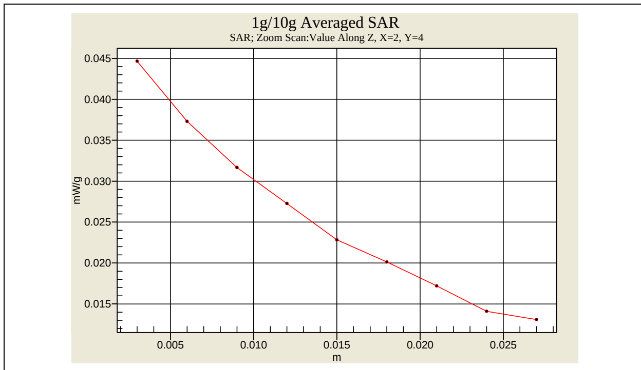
FRS Body SAR with Headset and Belt Clip _ CH11 (Ni-MH Battery)
