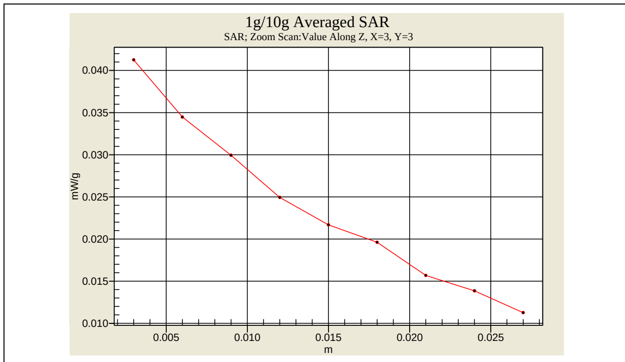
FRS Face SAR -15 mm Spacing _ CH11 (Ni-MH Battery)
