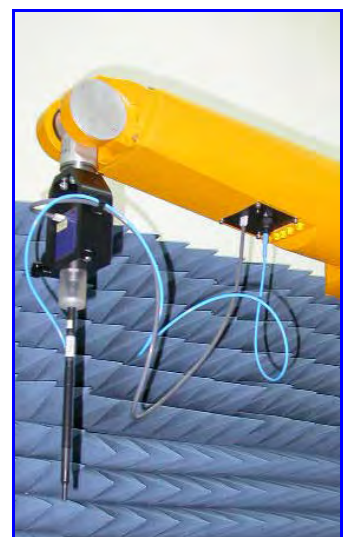
Figure 10. Probe setup on robot
