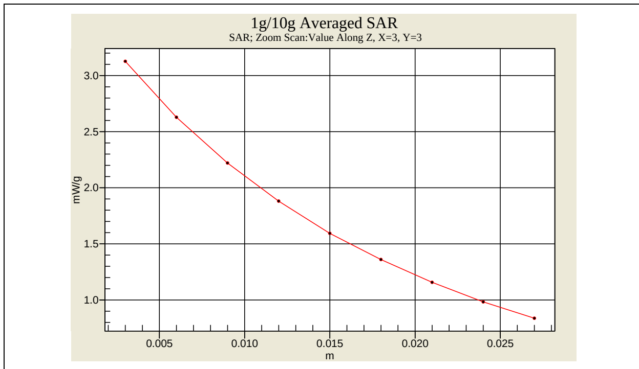
GMRS Face SAR - 15 mm Spacing _ CH4 (Ni-MH Battery)
