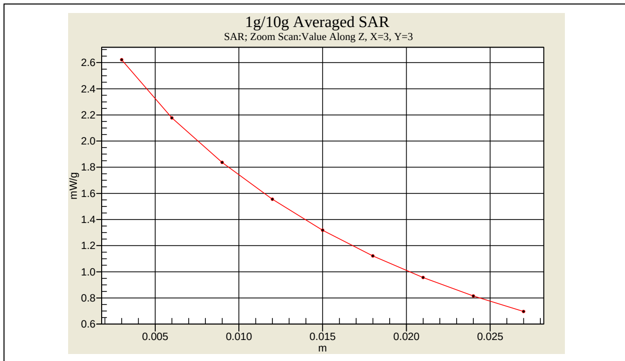
GMRS Body SAR with Headset and Belt Clip _ CH4 (ALKALINE Battery)
