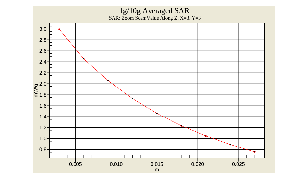
GMRS Body SAR - 15 mm Spacing _ CH4 (ALKALINE Battery)
