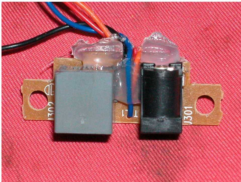
Base AC Adaptor Jack and Telephone Line Jack PCB front side
