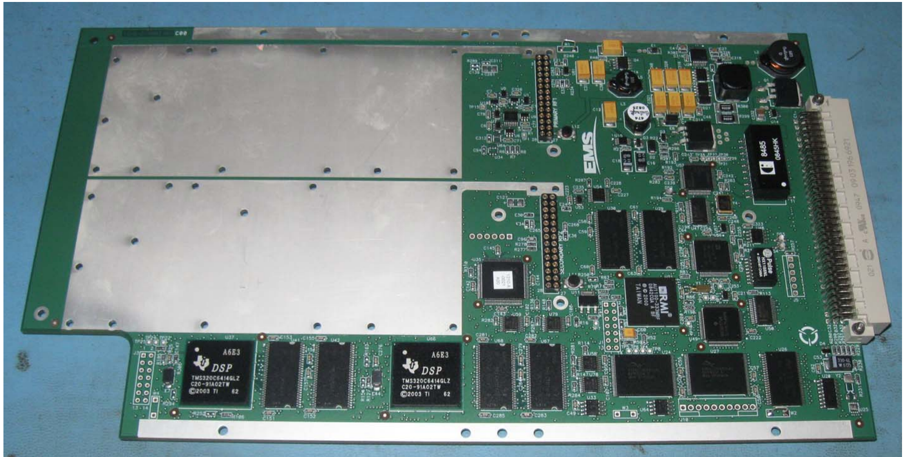
Figure 9: 1210-A-0002-01 HSD Digital Module Top (Part of the BGAN 2 Channel Card)
