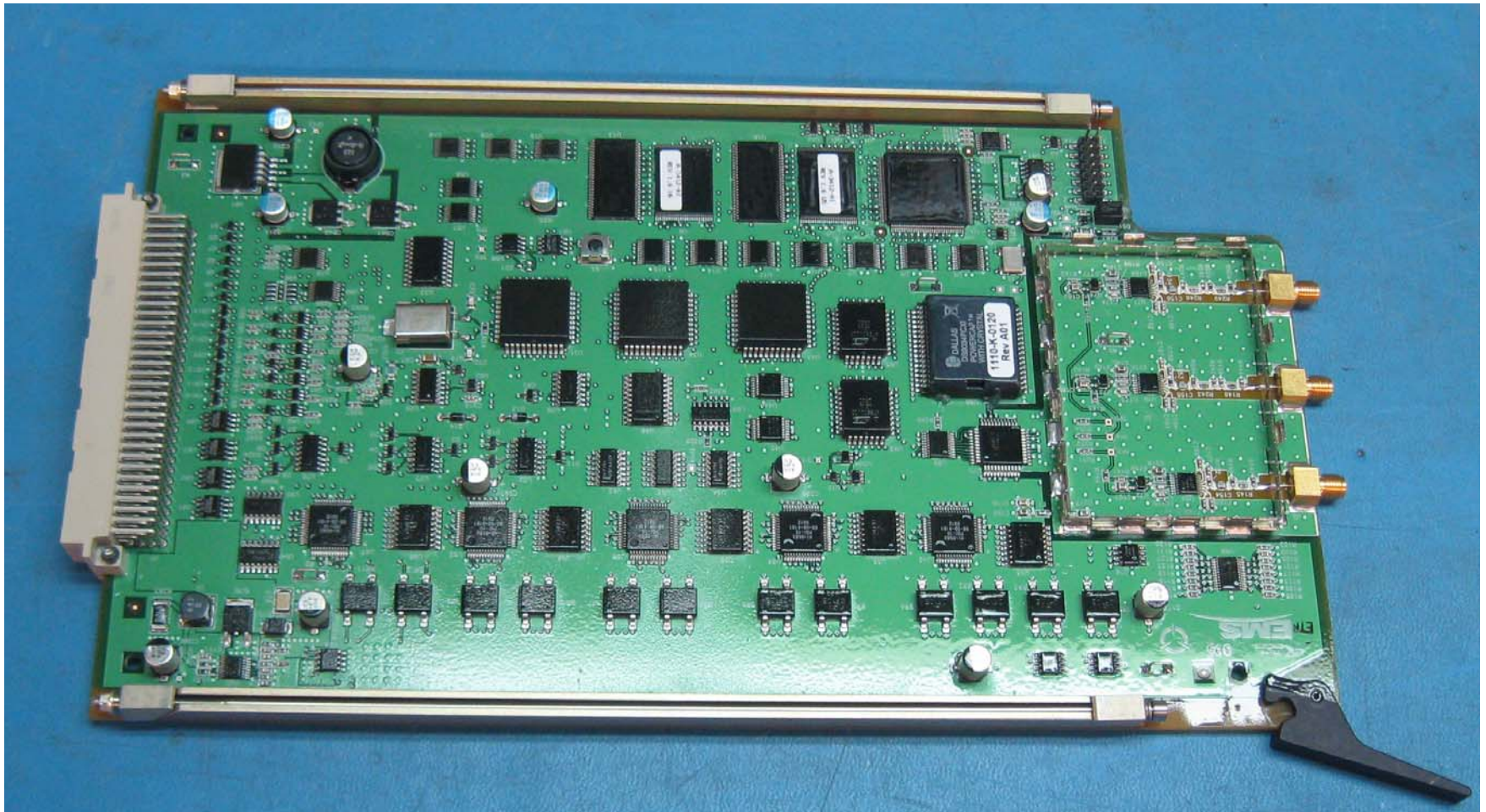
Figure 2: 1252-K-3411-01 Control Processor without Shield
