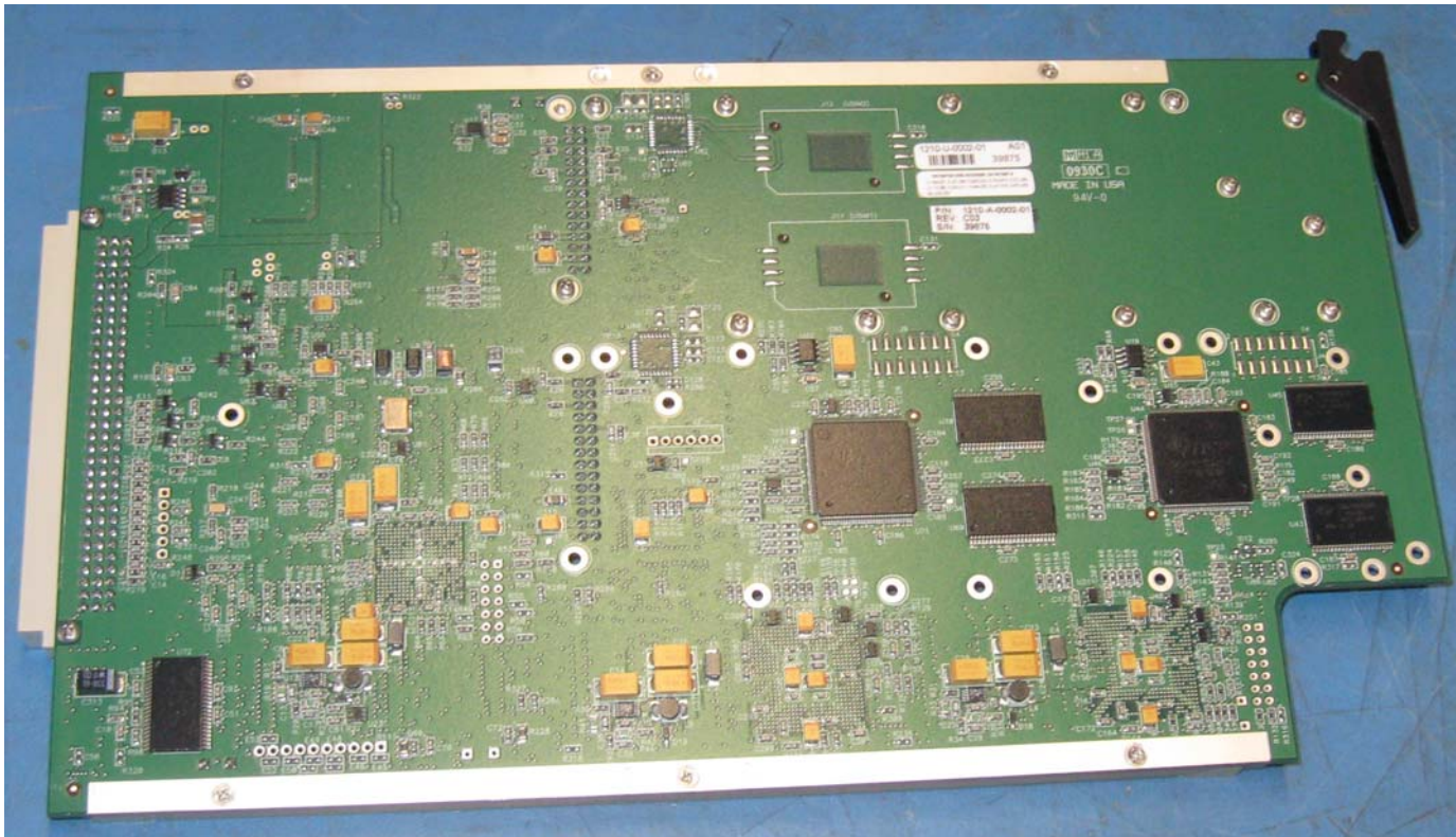
Figure 10: 1210-A-0002-01 HSD Digital Module Bottom (Part of the BGAN 2 Channel Card)
