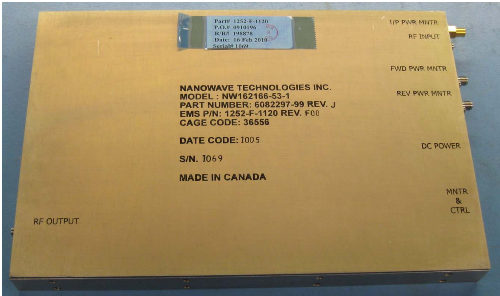
Figure 19: 1252-F-1120 HPA Bottom
