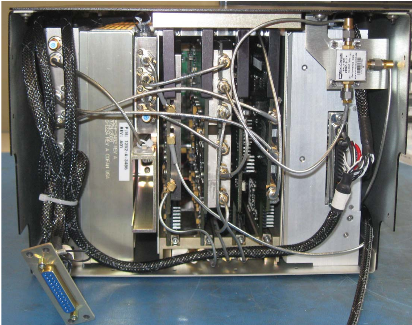
Figure 23: Interconnections
