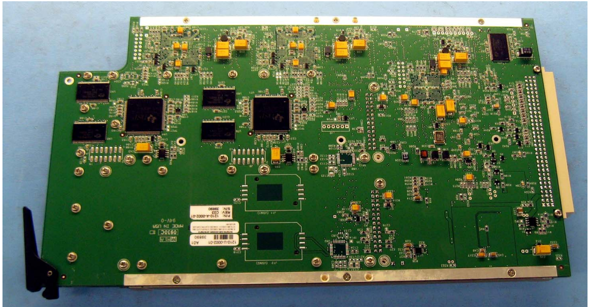
Figure 8: 1210-A-0010-02 BGAN 2 Channel Card Bottom
