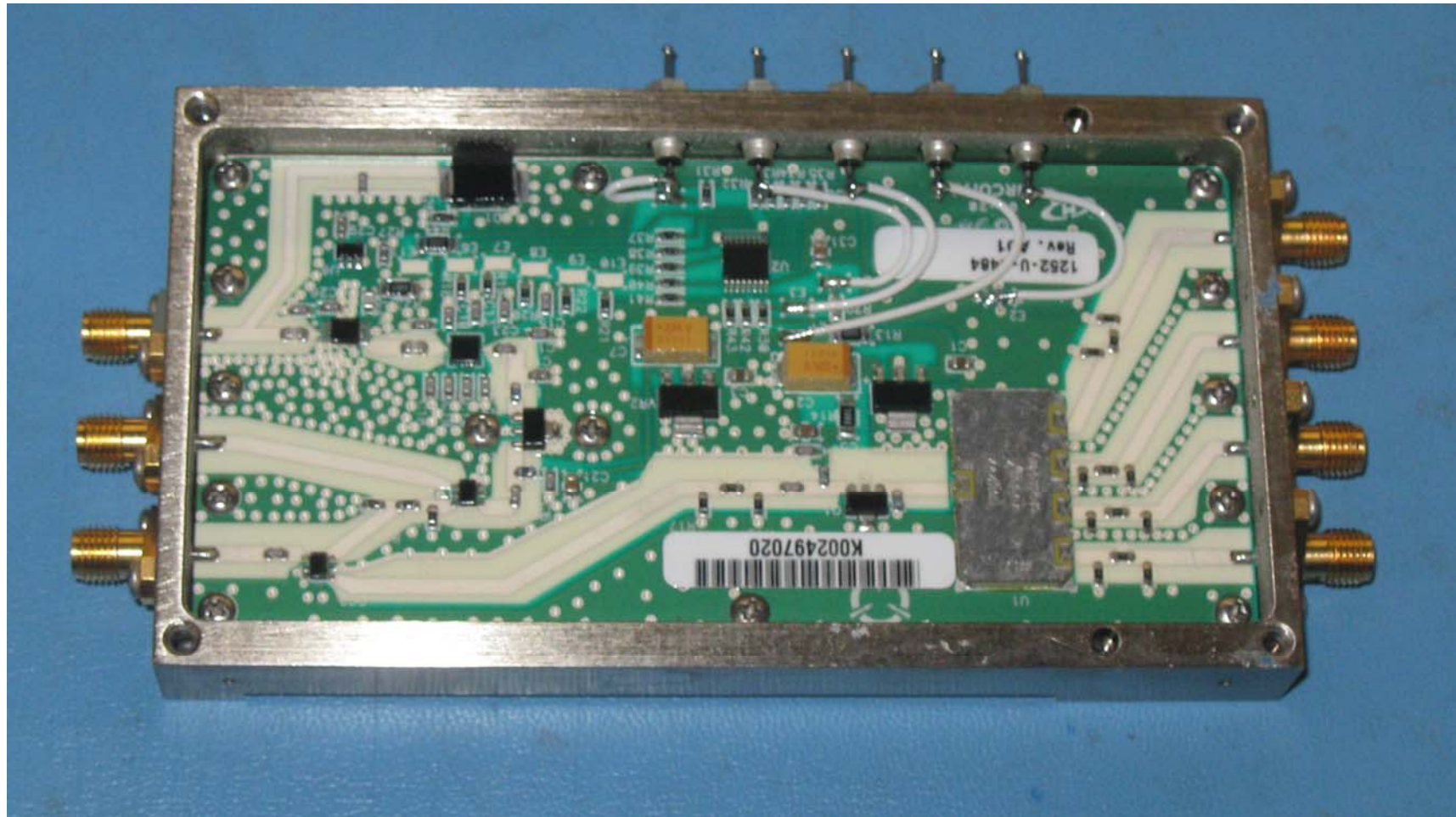
Figure 21: 1252-A-3439 RF Combiner Inside
