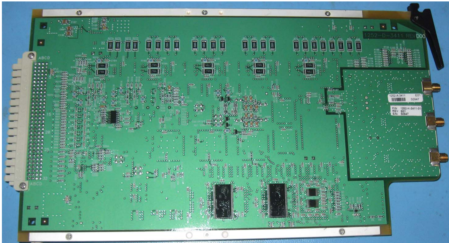
Figure 3: 1252-K-3411-01 Control Processor Bottom
