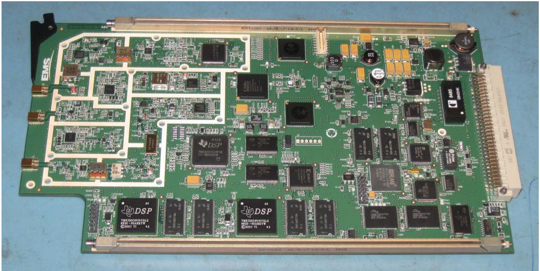
Figure 5: 1210-A-1510 HSD Multi Channel Card without Shield
