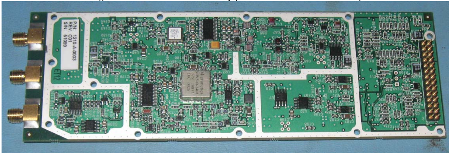
Figure 12: 1210-A-0003 RF Module Bottom (Part of the BGAN 2 Channel Card)
