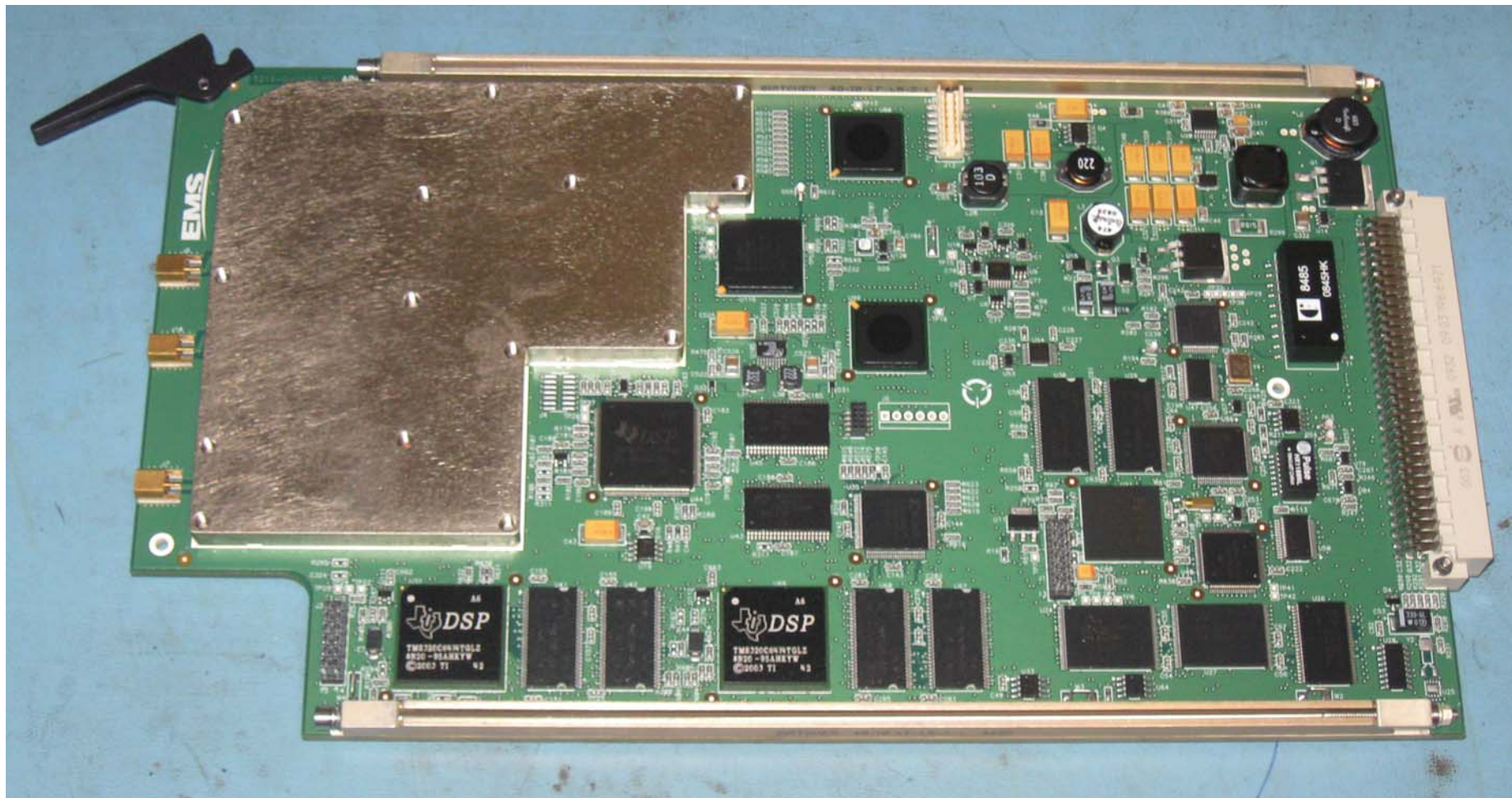
Figure 4: 1210-A-1510 HSD Multi Channel Card Top
