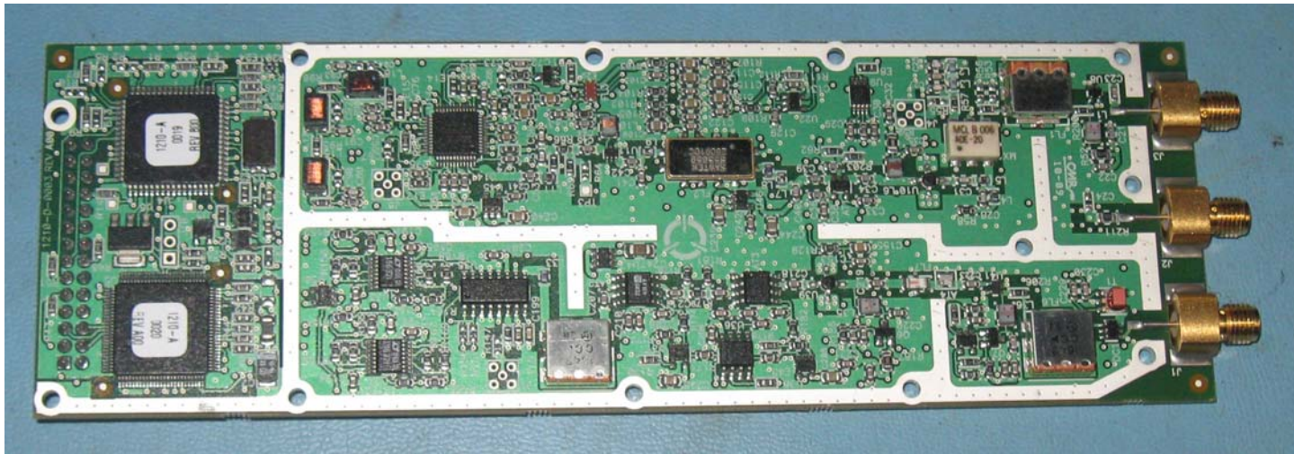
Figure 11: 1210-A-0003 RF Module Top (Part of the BGAN 2 Channel Card)
