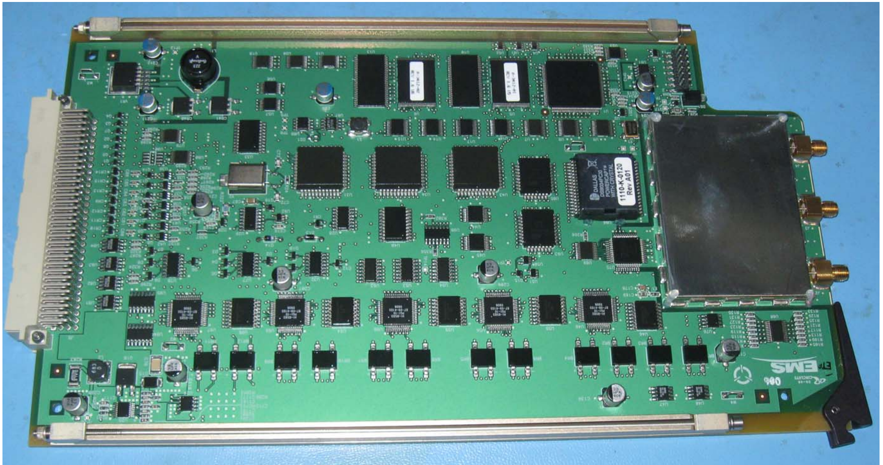
Figure 3: Control Processor with Shield Top
