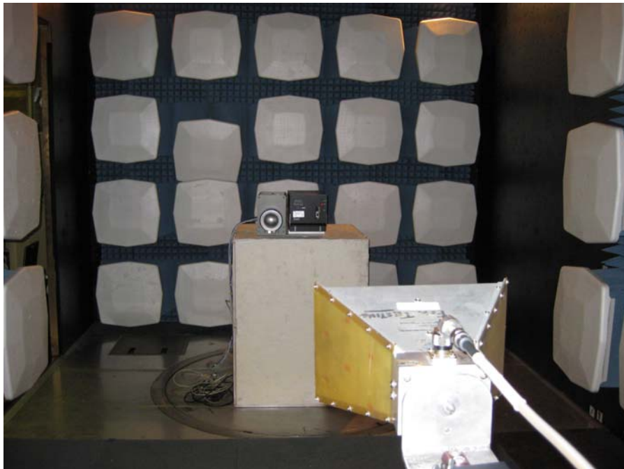
Radiated #2
