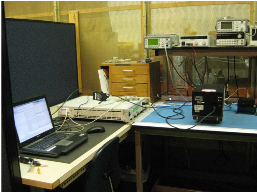
Conducted #2
