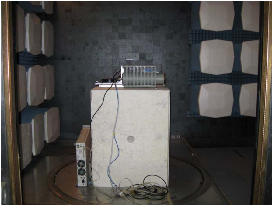
Radiated
