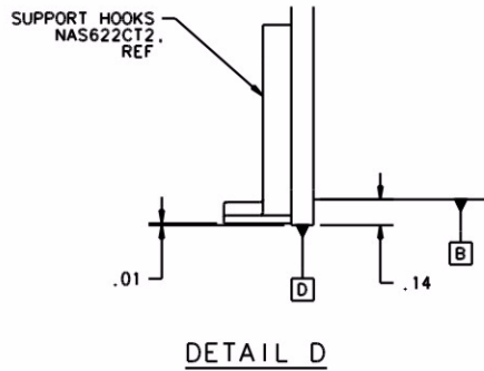
Figure 3-1 ARINC 781 SDU Outline and Installation Drawing, 1394-E-1100 Rev B00 (Sheet 1 of 2)
