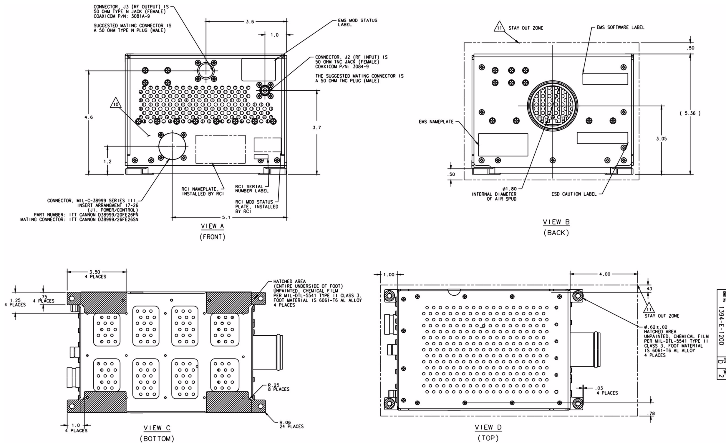
Figure 3-4 ARINC 781 FMPA Outline and Installation Drawing, 1394-E-1200 Rev D00 (Sheet 2 of 2)
