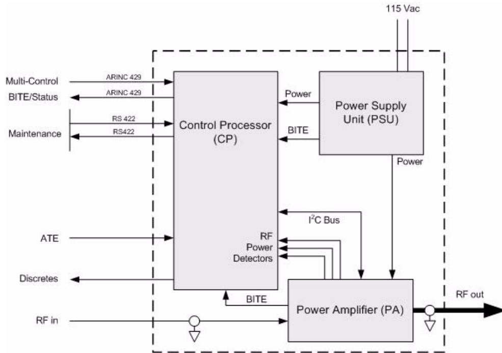
Figure 1-4 FMFA Block Diagram
