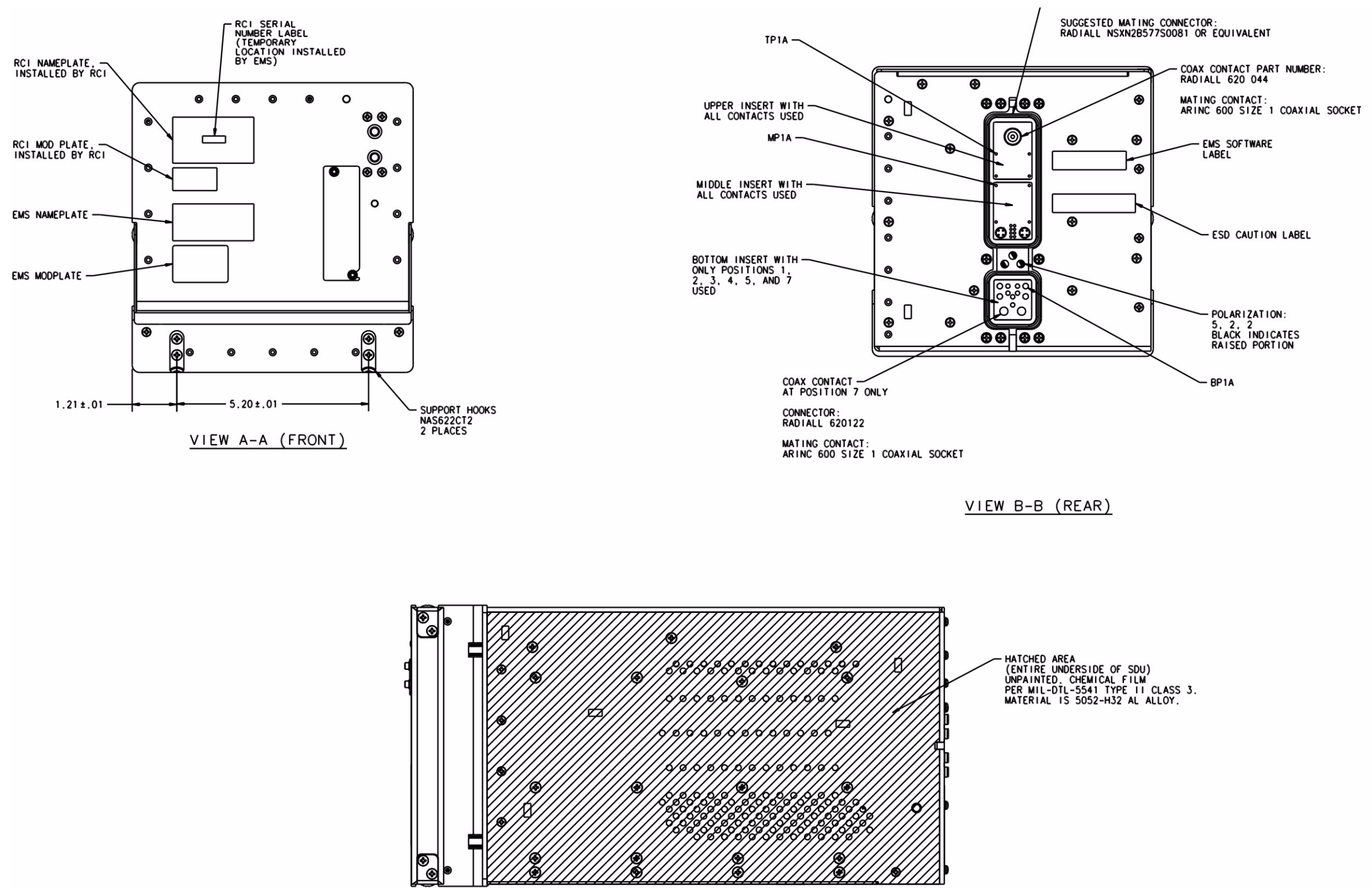
Figure 3-2 ARINC 781 SDU Outline and Installation Drawing, 1394-E-1100 Rev B00 (Sheet 2 of 2)
