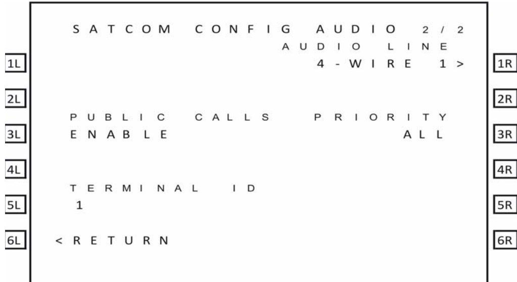
Figure 2-13 CONFIG AUDIO 2/2
