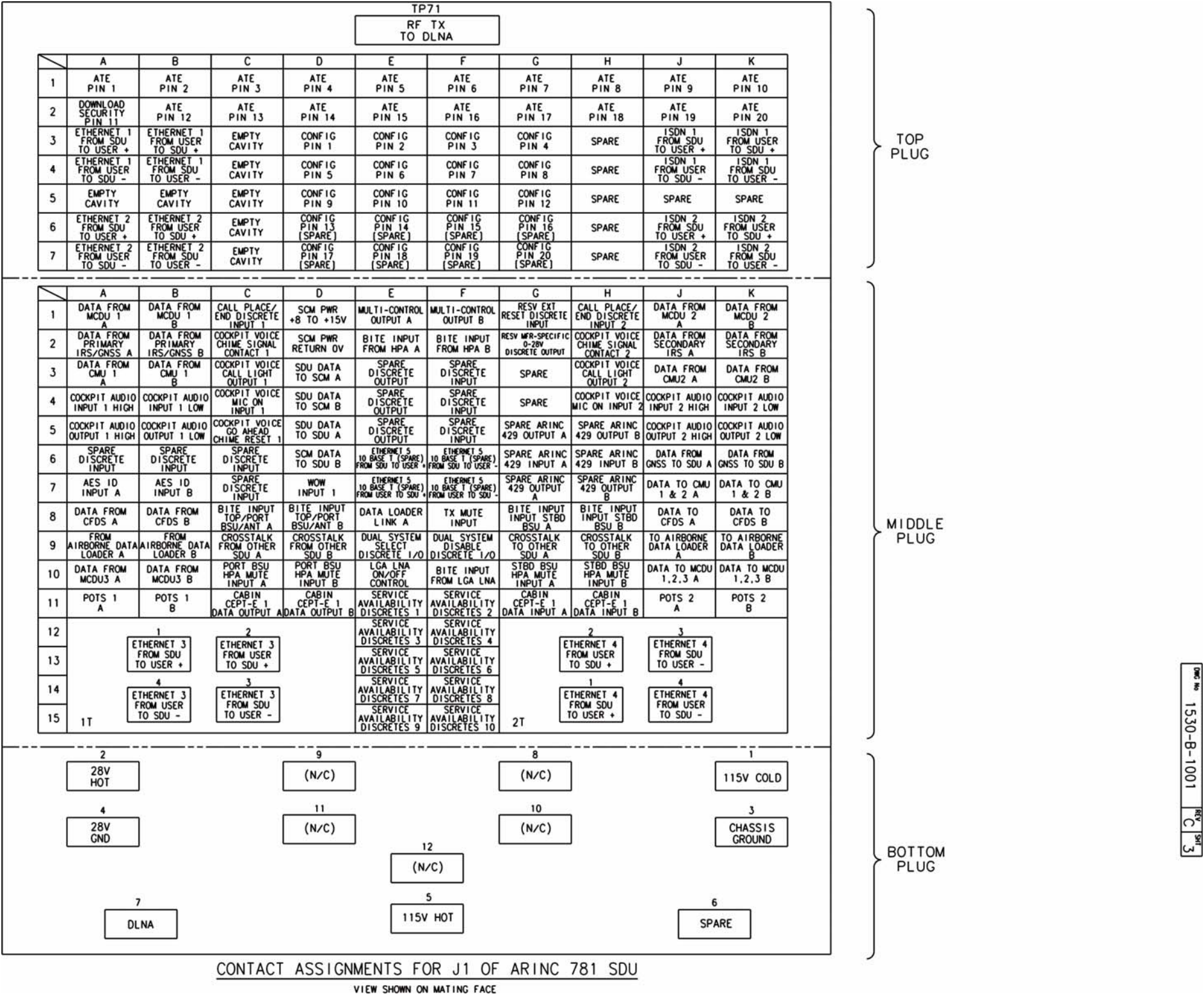
Figure 3-9 ARINC 781-200 System Interconnect Drawing, 1530-B-1001 Rev C00 (Sheet 3 of 3)
