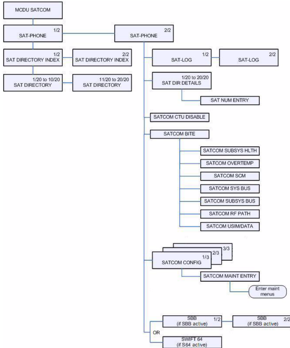
Figure 2-2 A781-200 MCDU Menu Structure
