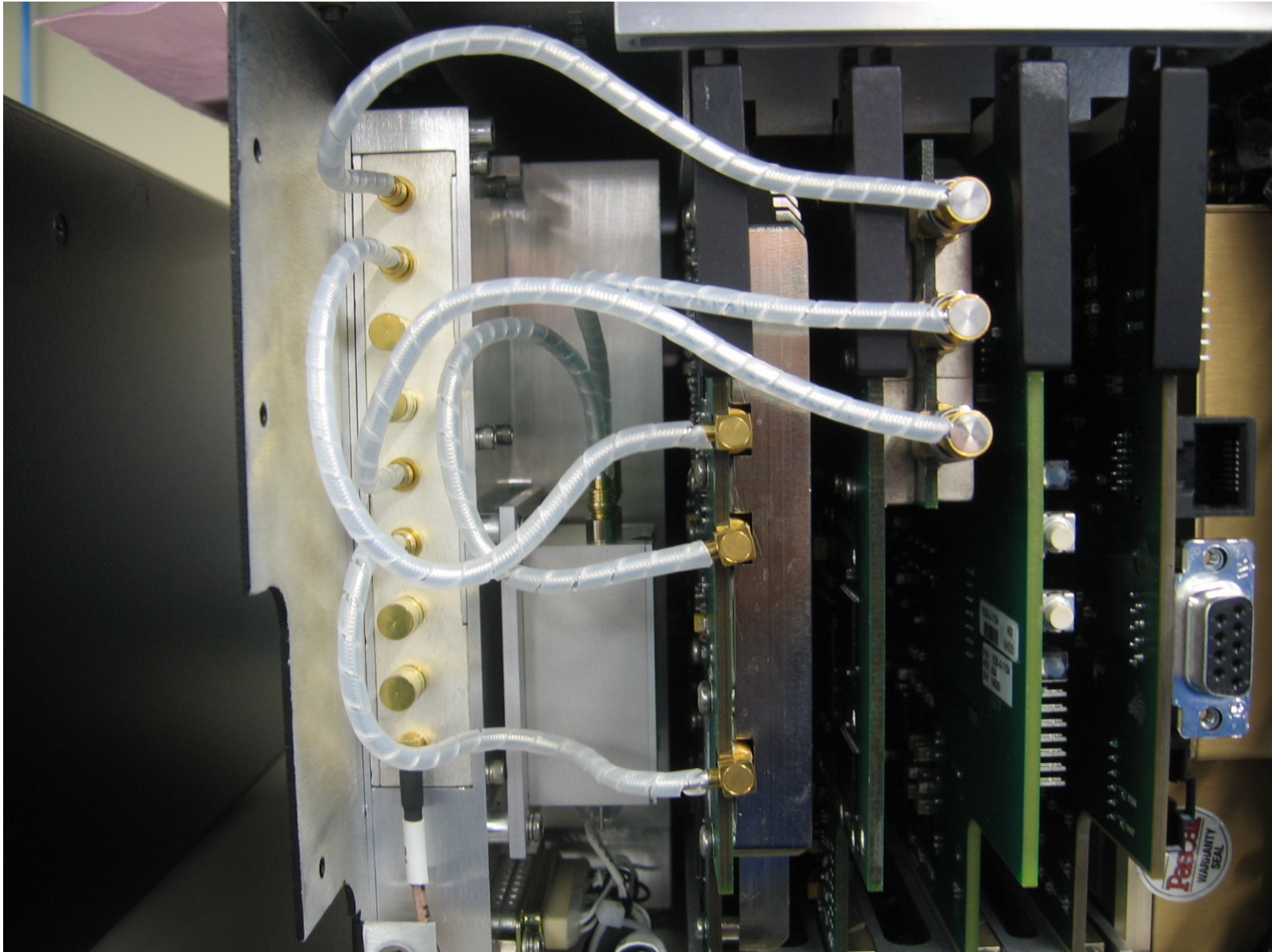
Figure 19: Interconnections
