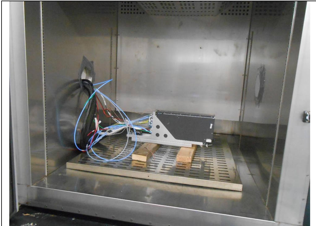
Frequency Stability #2
