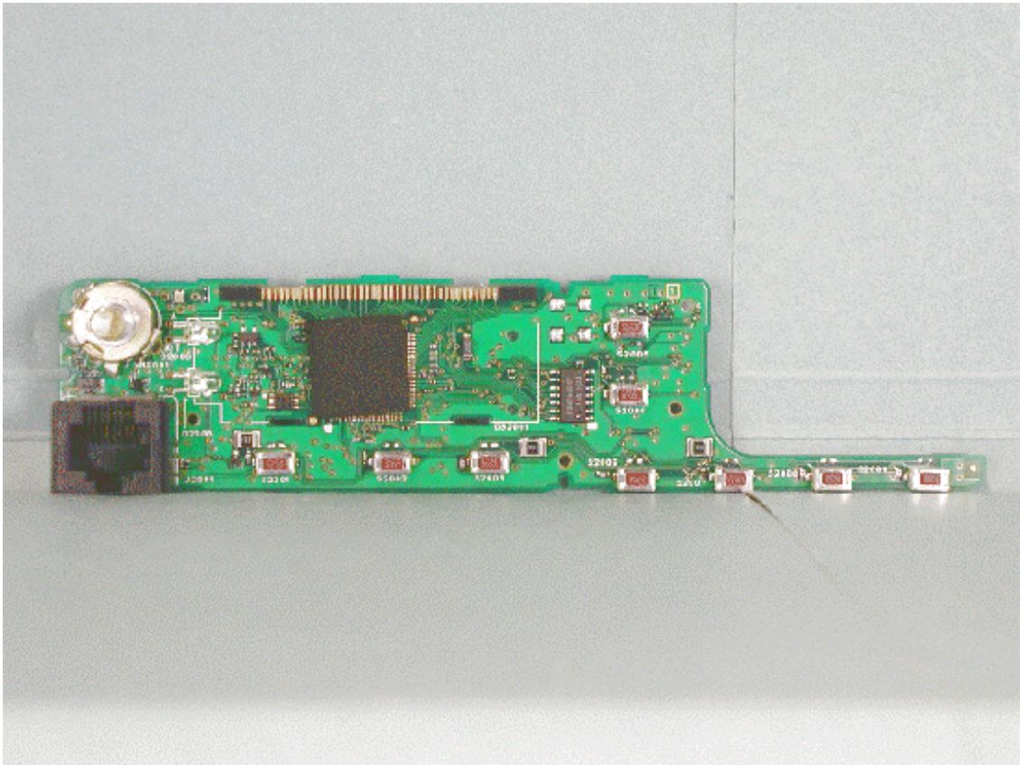
Side-A of PANEL-UNIT without LCD
