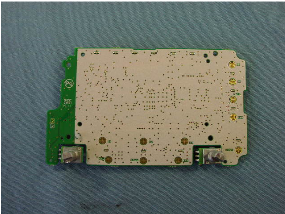
Side-A of CNTL-2 UNIT without LCD (GX1700)
