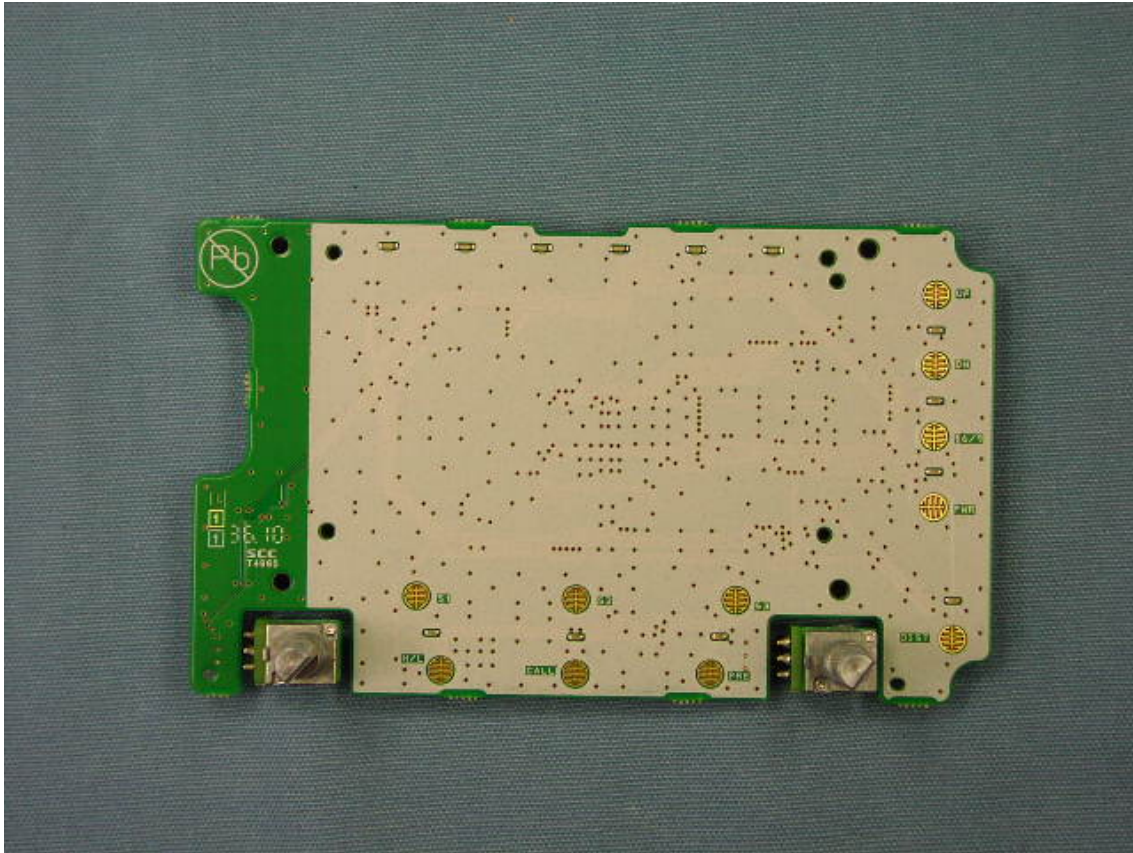
Side-A of CNTL-UNIT without LCD (GX1600)
