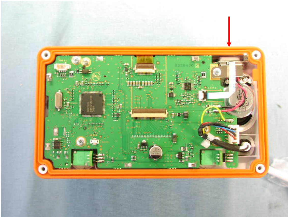
Back of Front Panel with GPS-UNIT (GX1700)
