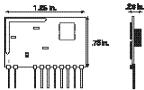
Figure 10: Physical package
