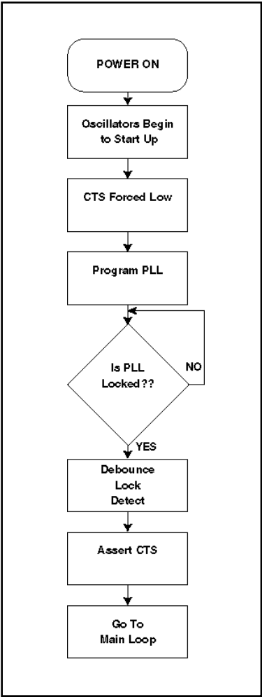
Figure 16: Start-up sequence
