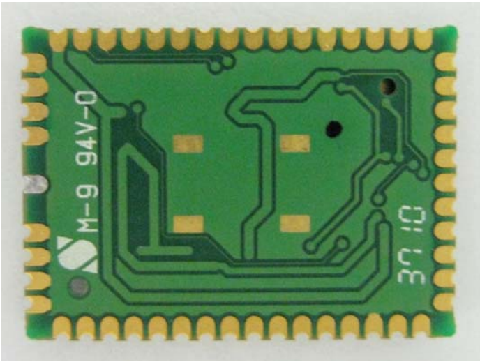
Back side of module
