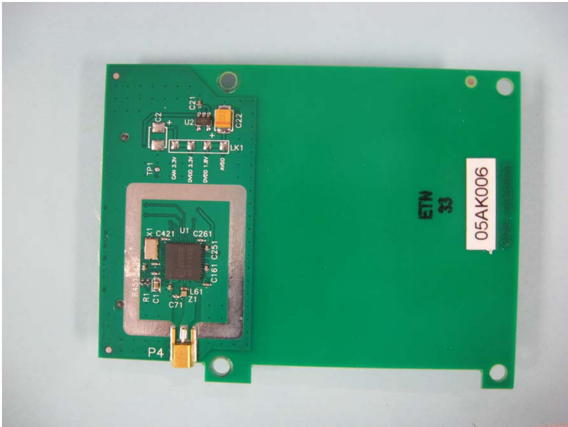
Anaren Radio Board Top View
