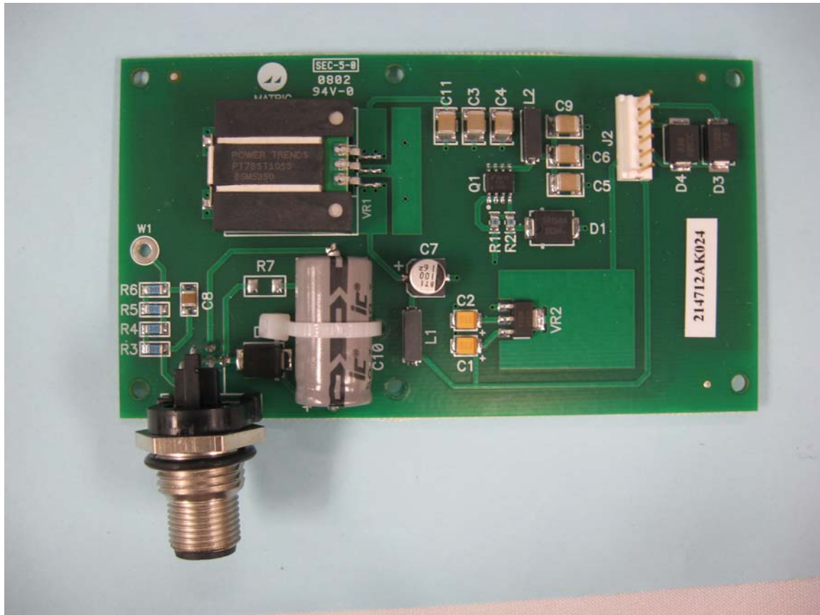
Power Board Top View
