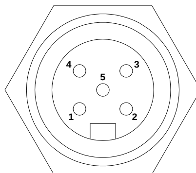
Male (pins)
