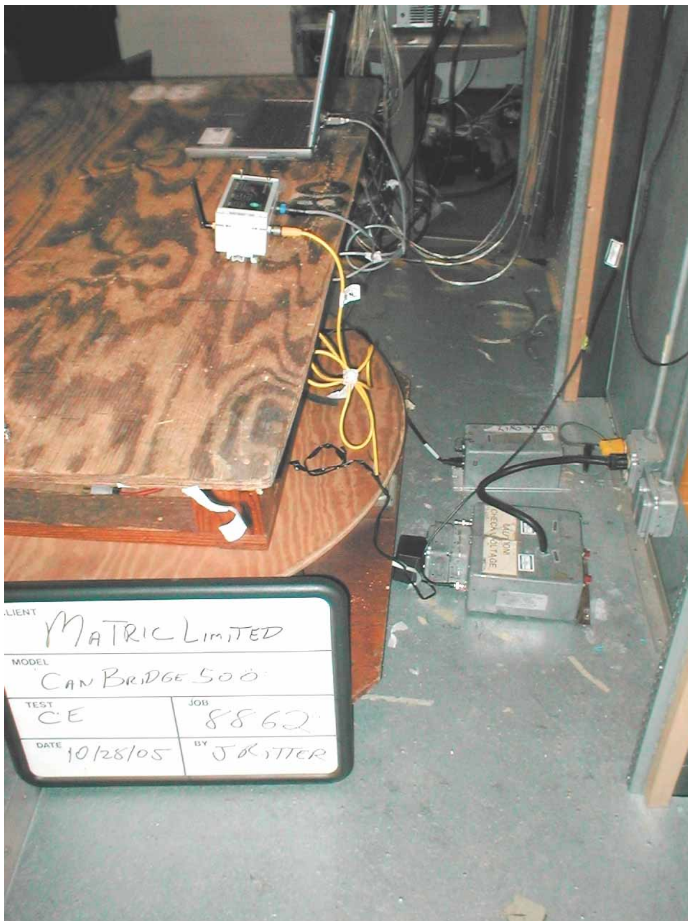
Conducted Emissions Test Setup, Photograph #2
