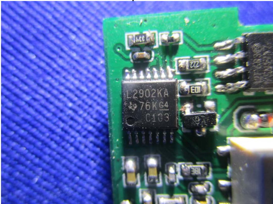
Chip View
