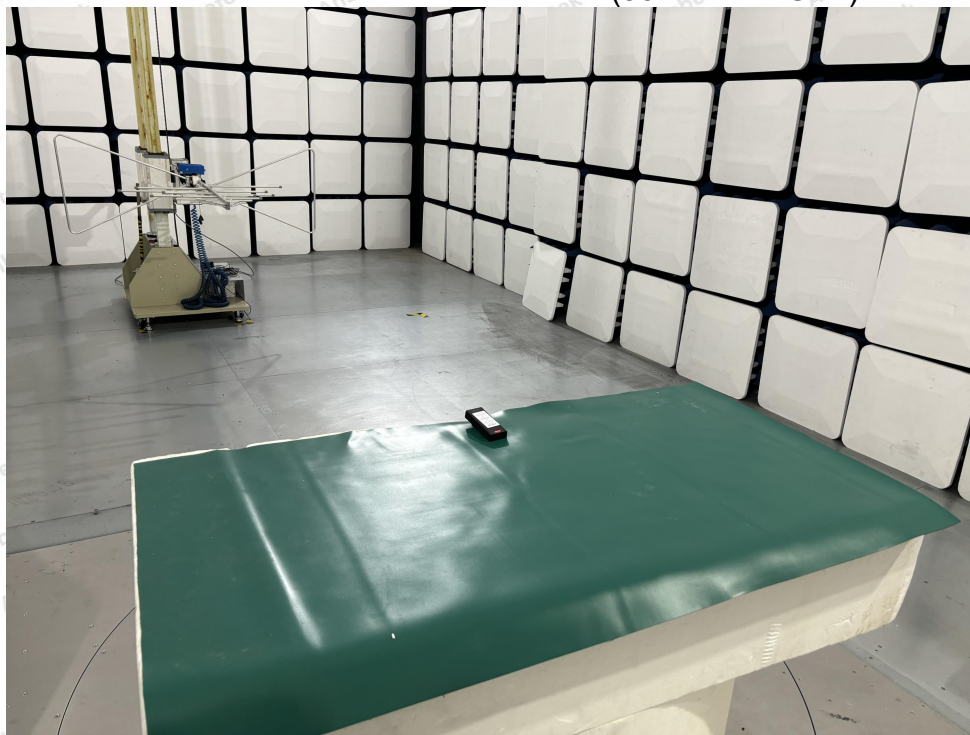
Photo of Radiation Emission Test (30MHz to 1GHz)
