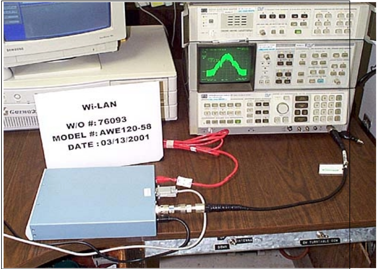
Antenna Conducted - 5MHz - 1GHz and Fundamental
