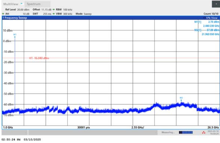
BLE_2M-Ant1-2480-1000~26500-PASS
