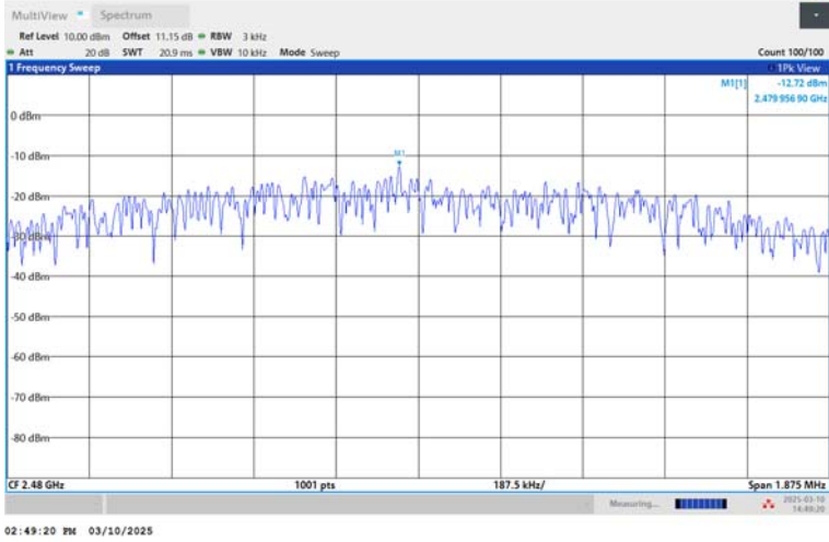
BLE_2M-Ant1-2480-PASS
