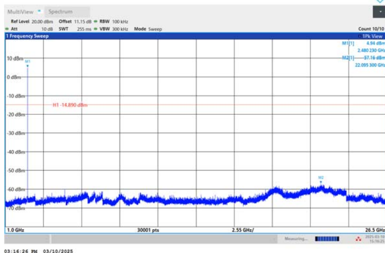
3DH5-Ant1-2480-1000~26500-PASS
