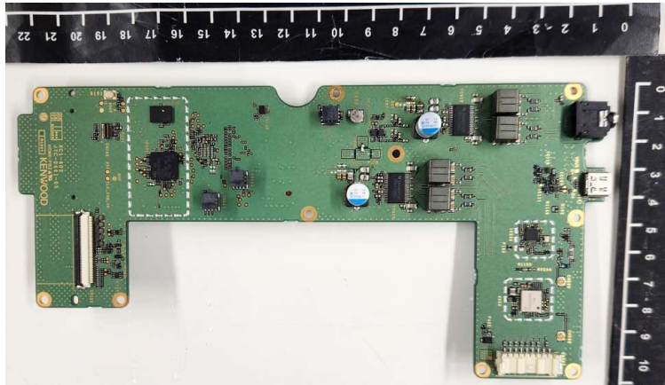
CONT UNIT without shield case - side A
