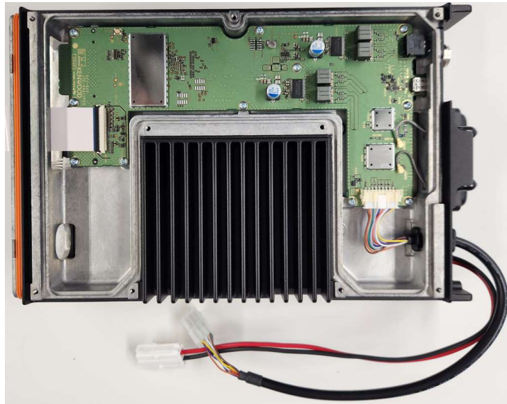
Top Internal View of CONT Unit
