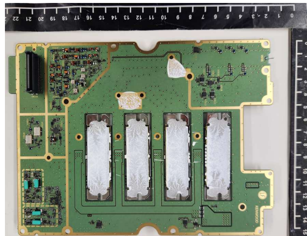
RF Unit with shield case - side B -
