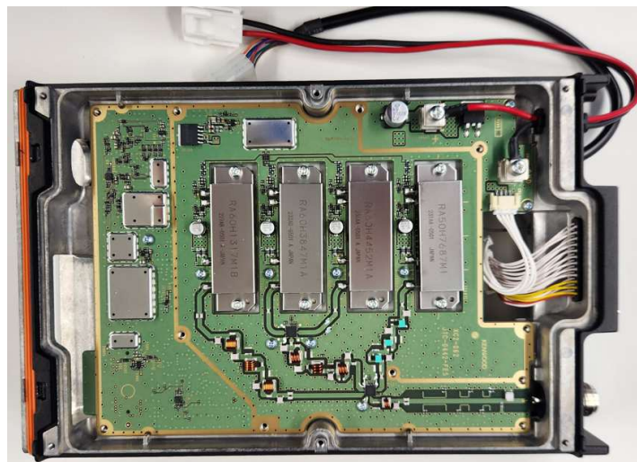
Bottom Internal View of RF Unit
