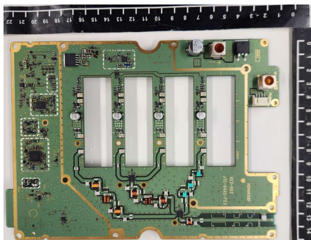
RF Unit without shield case - side A -
