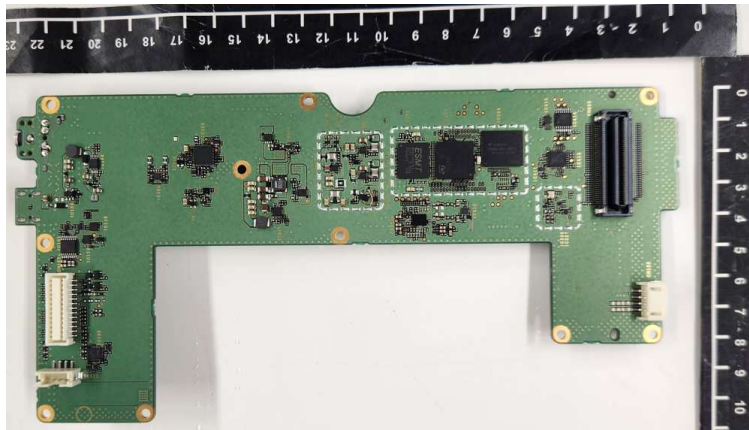
CONT UNIT without shield case - side B -
