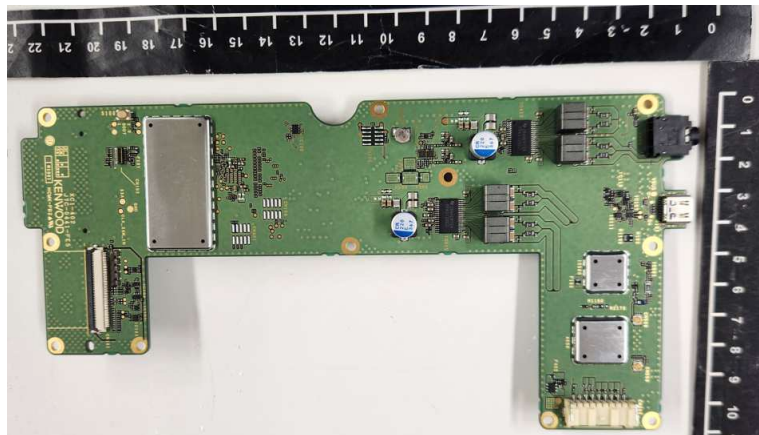
CONT Unit with shield case - side A -
