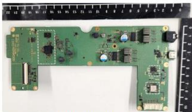
CONT UNIT without shield case - side A
