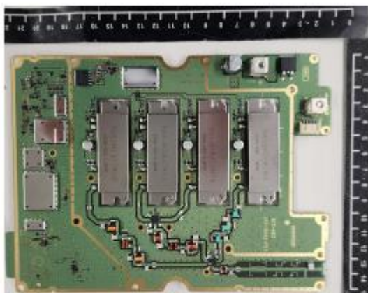
RF Unit with shield case - side A -
