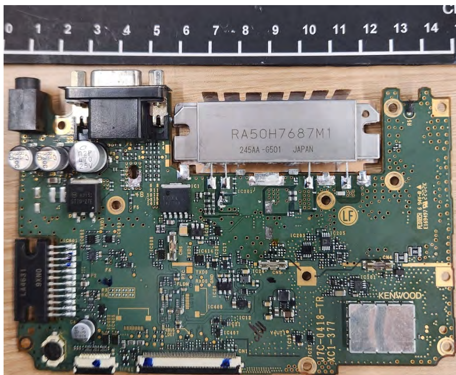
Upper side of TX-RX Unit
