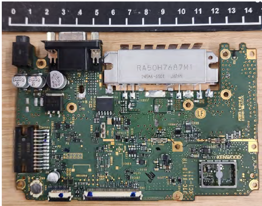
Upper side of TX-RX Unit (without shield case)
