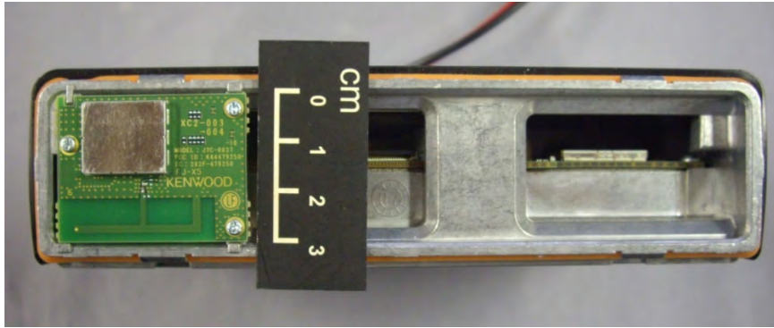
Front Internal View of Certificated Bluetooth Module
