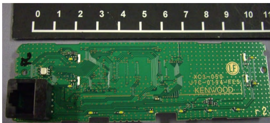
Bottom side of SUB Unit
