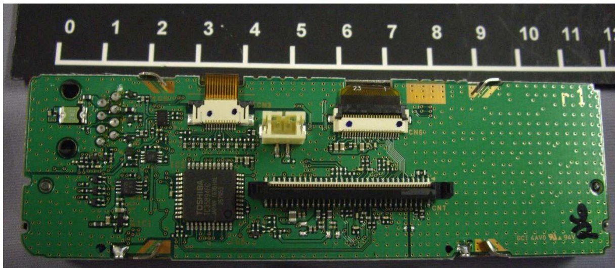
Upper side of SUB Unit
