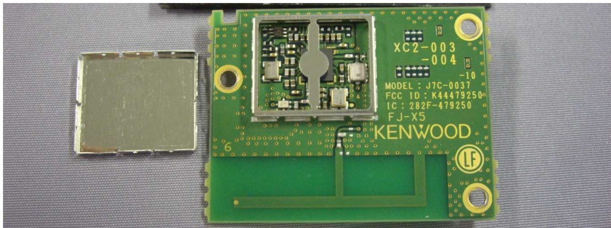
Upper side of Certificated Bluetooth Module (without shield case)
