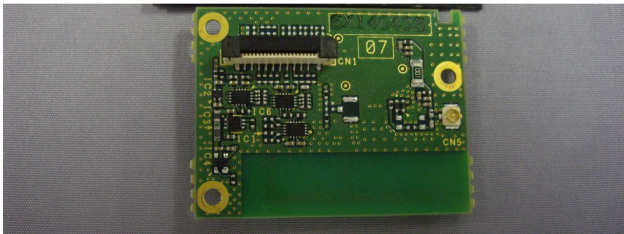
Bottom side of Certificated Bluetooth Module
