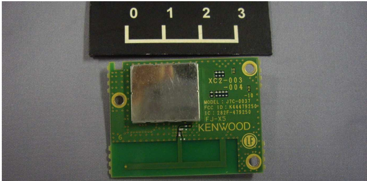
Upper side of Certificated Bluetooth Module (FCC ID: K44479250, IC: 282F-479250, MODEL: J7C-0037)
