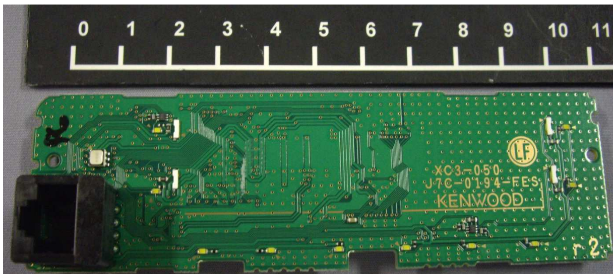
Bottom side of SUB Unit
