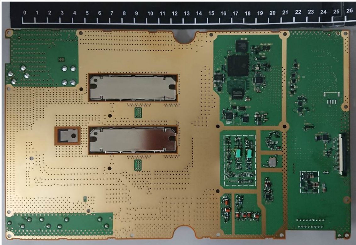
MAIN UNIT
