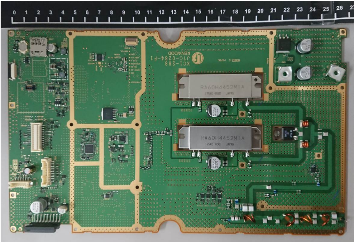
MAIN UNIT
