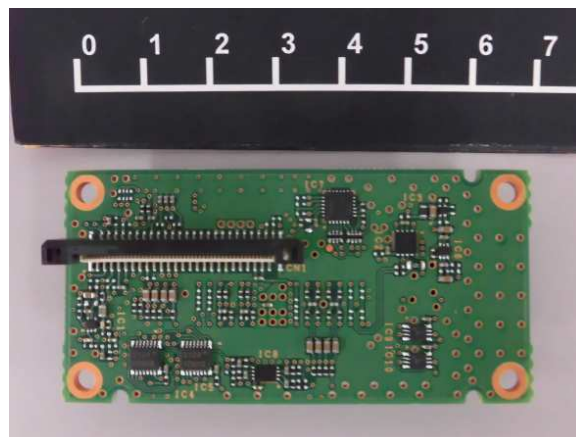
INTERFACE UNIT
