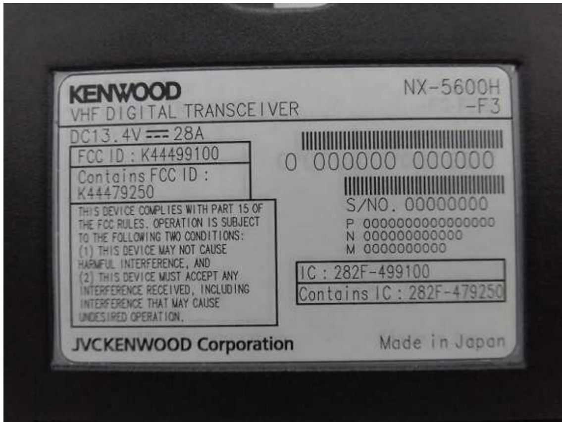
NX-5600H-F3 Name Plate
