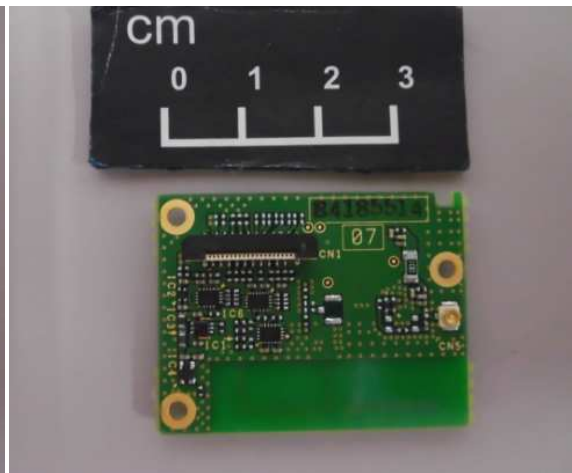
Certificated Bluetooth Module (FCC ID: K44479250, IC: 282F-479250, MODEL: J7C-0037)
