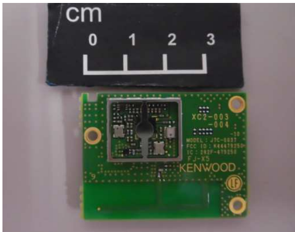
Certificated Bluetooth Module (FCC ID: K44479250, IC: 282F-479250, MODEL: J7C-0037)
