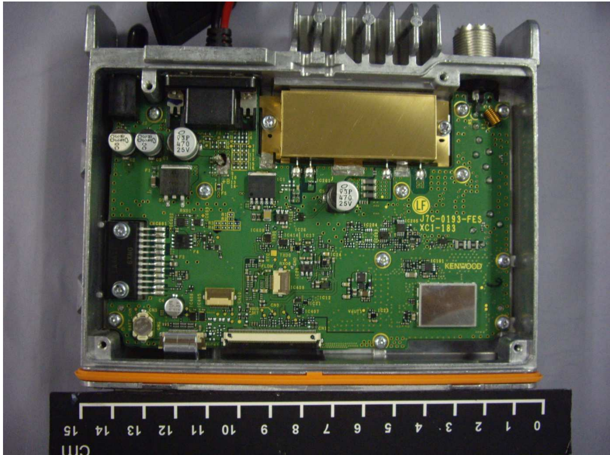
Top Internal View of TX-RX Unit
