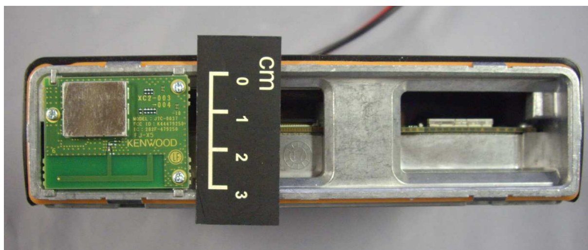
Front Internal View of Certificated Bluetooth Module
