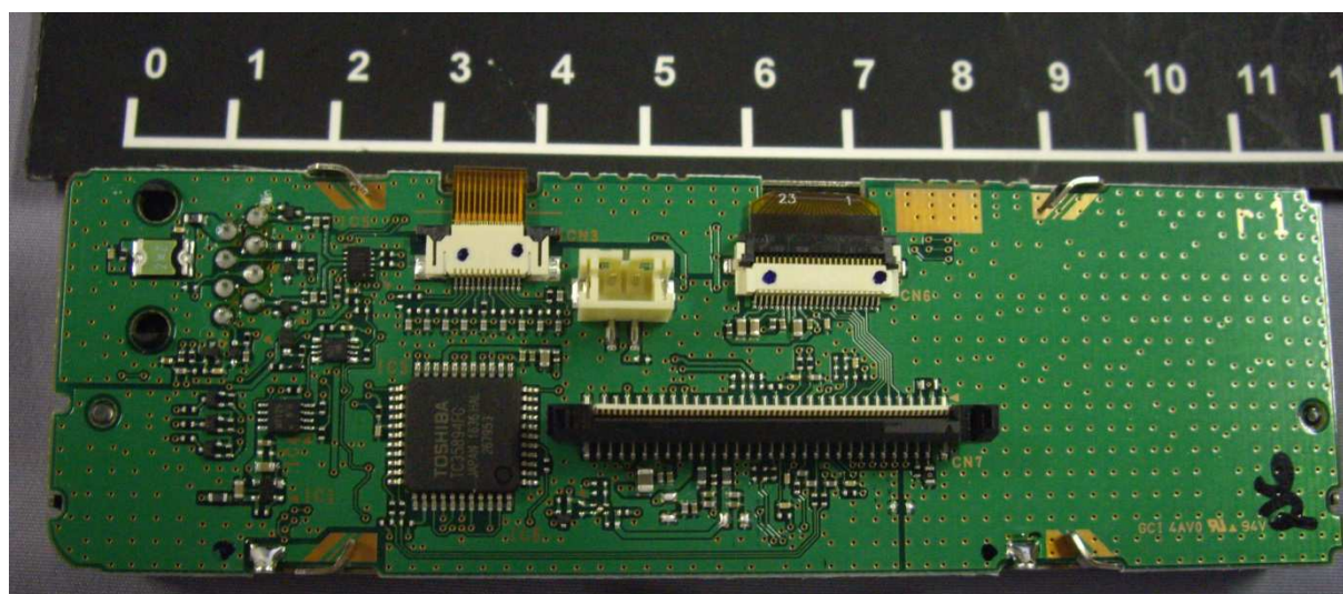
Upper side of SUB Unit
