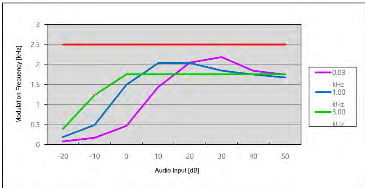
11K0F3E_470.05 MHz_LOW POWER
