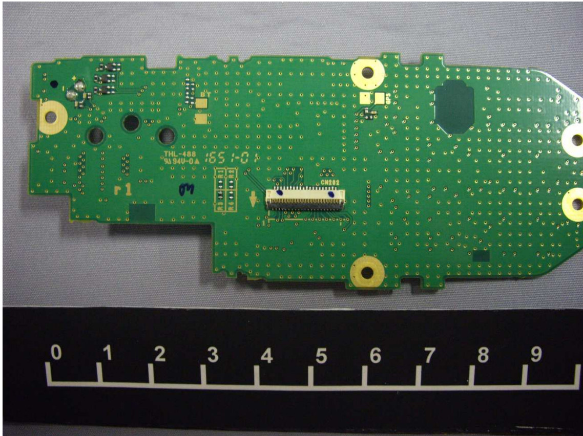
DISPLAY Unit of NX-3220-K (Bottom)
