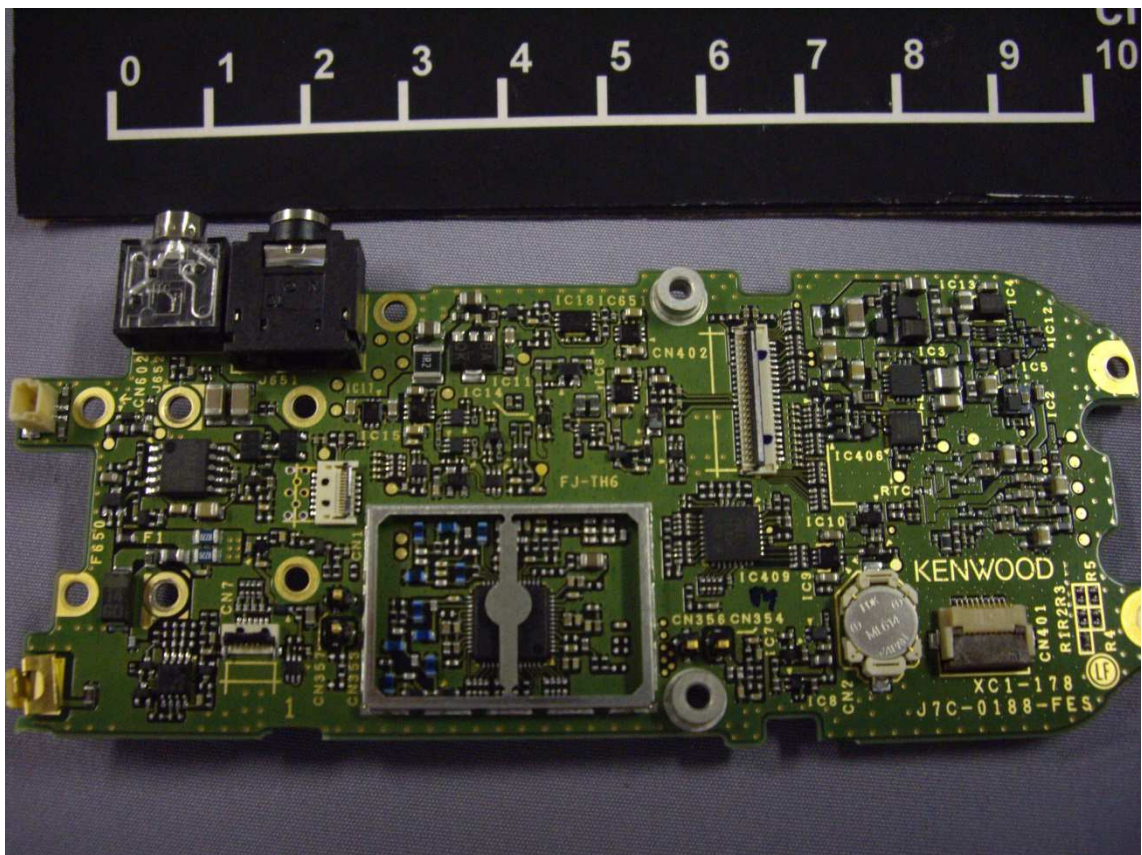
TX-RX Unit of NX-3220-K_K2_K3 without shield case (Top)
