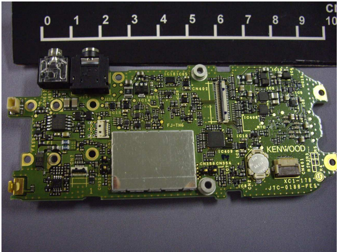
TX-RX Unit of NX-3220-K_K2_K3 (Top)
