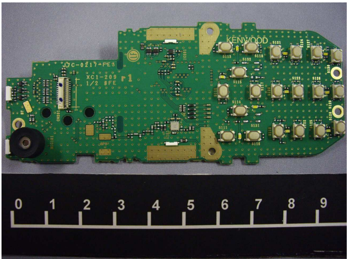
DISPLAY Unit without LCD of NX-3220-K3 (Top)
