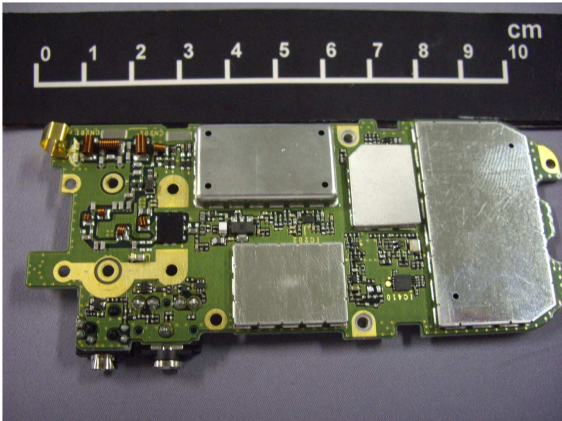
TX-RX Unit of NX-3220-K_K2_K3 (Bottom)
