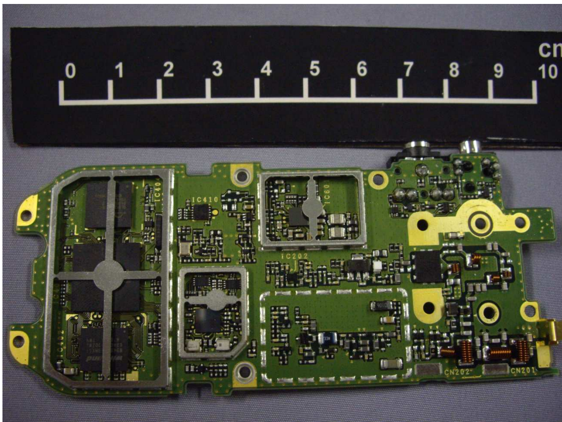
TX-RX Unit of NX-3220-K_K2_K3 without shield case (Bottom)
