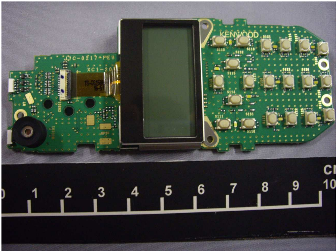
DISPLAY Unit of NX-3220-K3 (Top)
