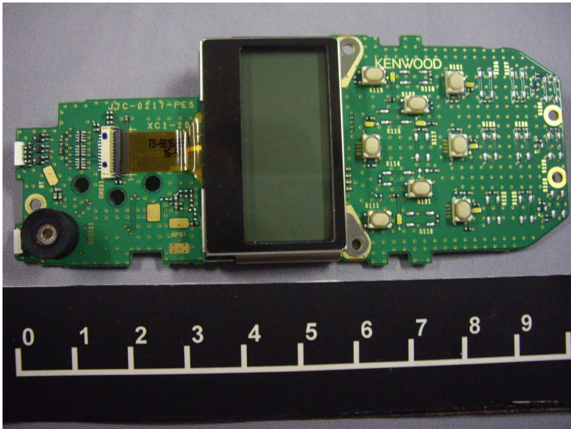
DISPLAY Unit of NX-3220-K2 (Top)
