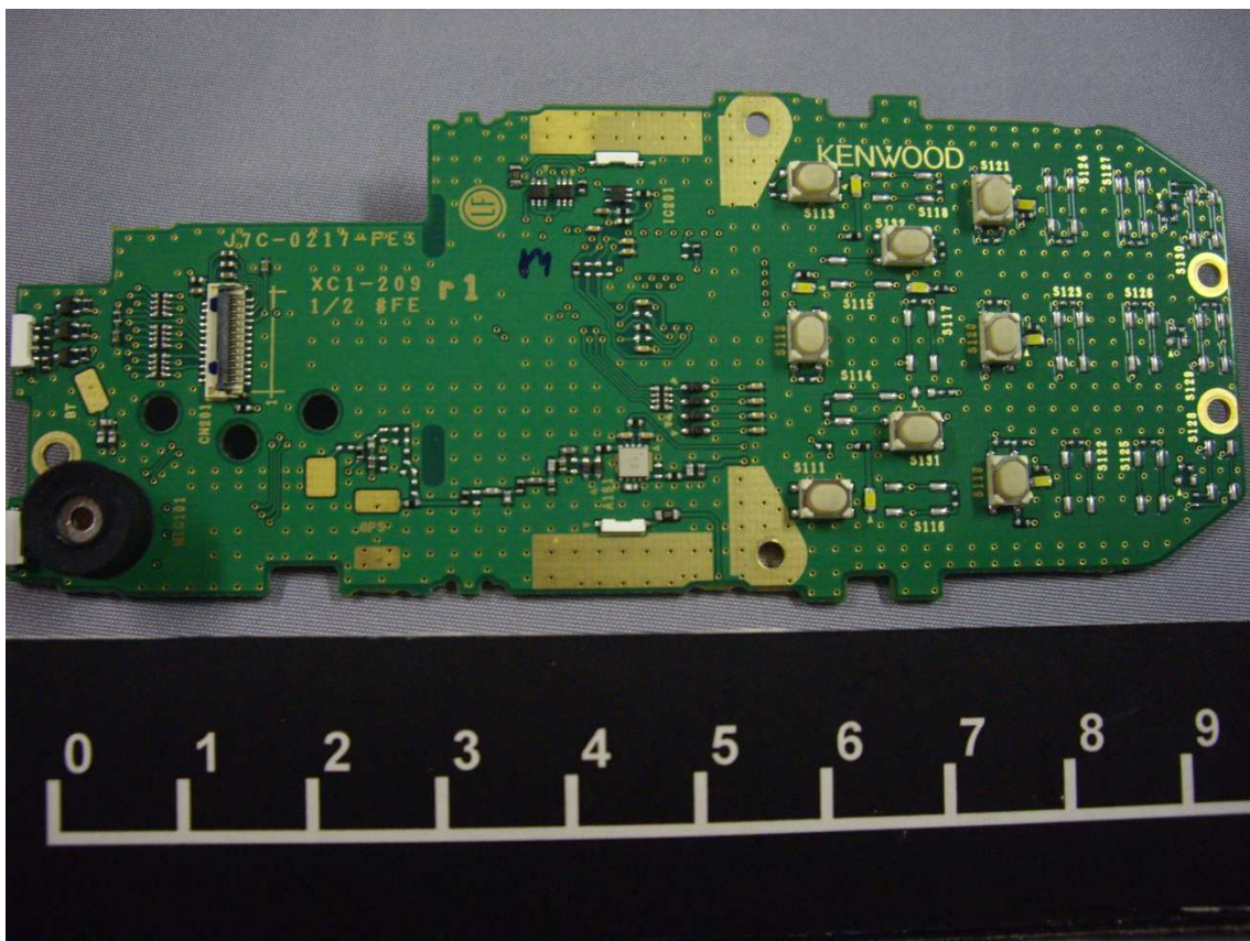
DISPLAY Unit without LCD of NX-3220-K2 (Top)
