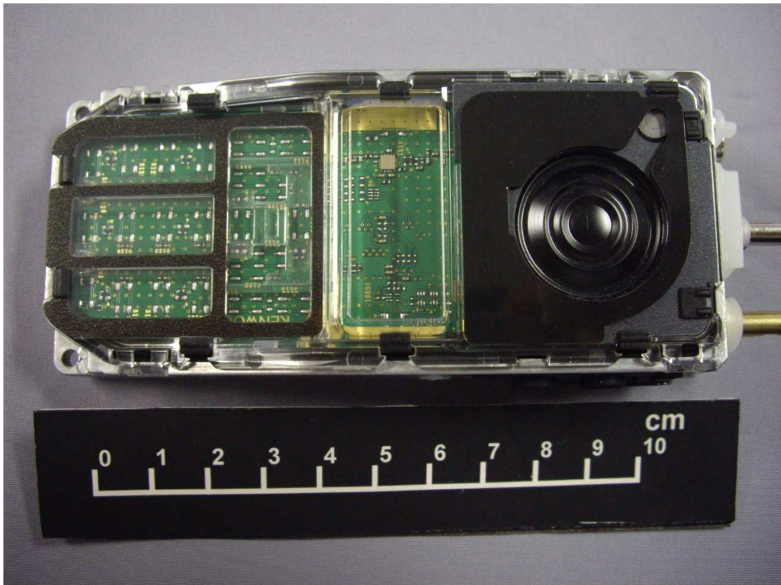
Top Internal View of NX-3220-K
