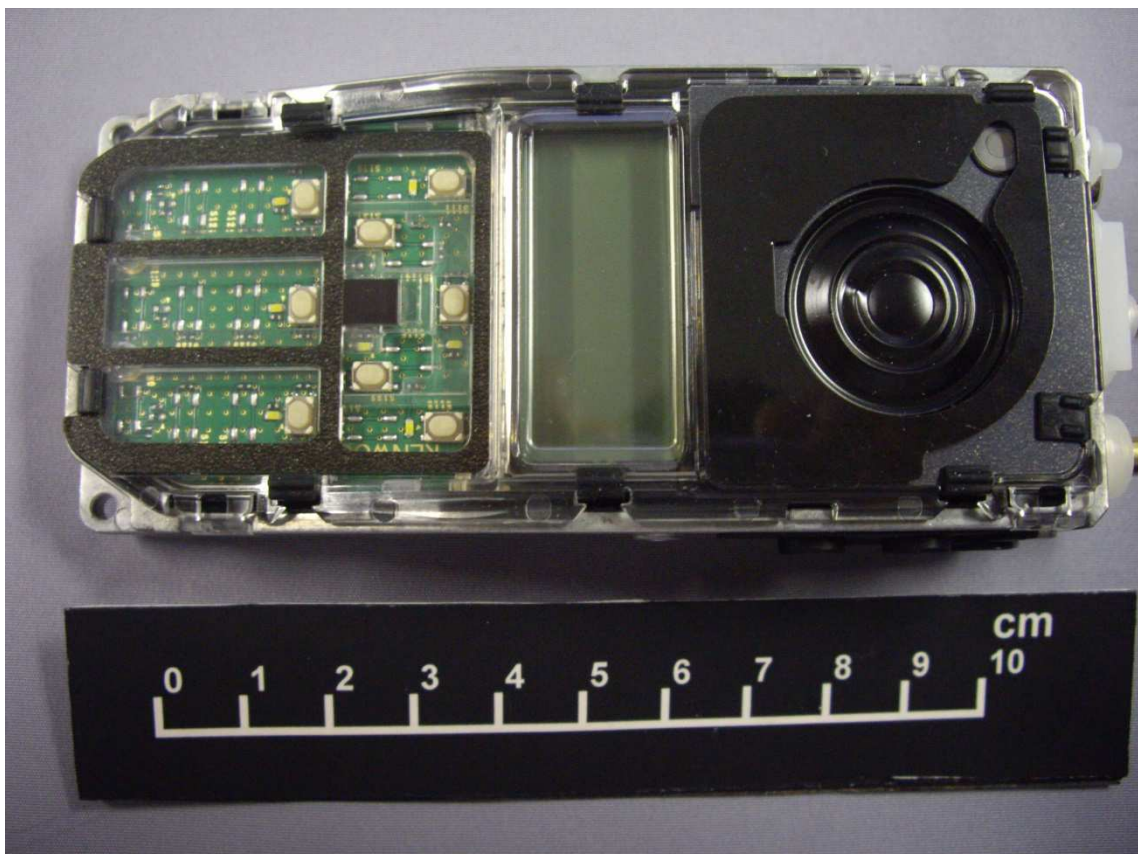
Top Internal View of NX-3220-K2
