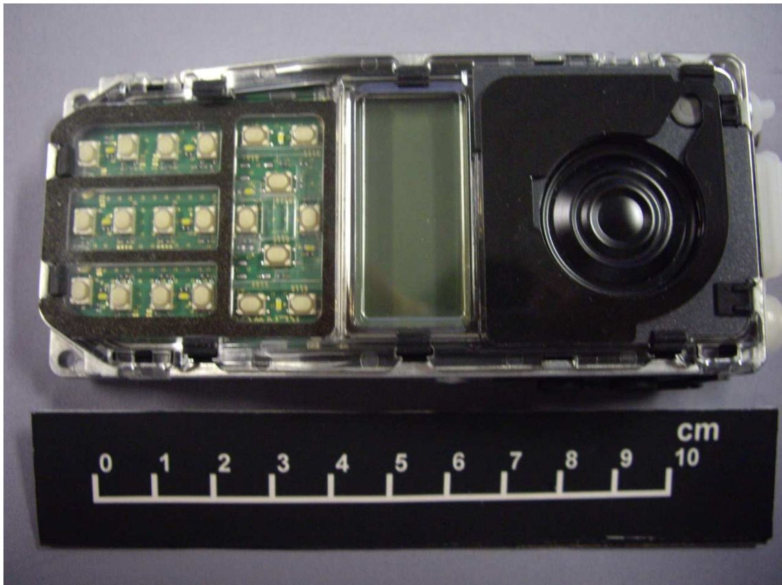
Top Internal View of NX-3220-K3
