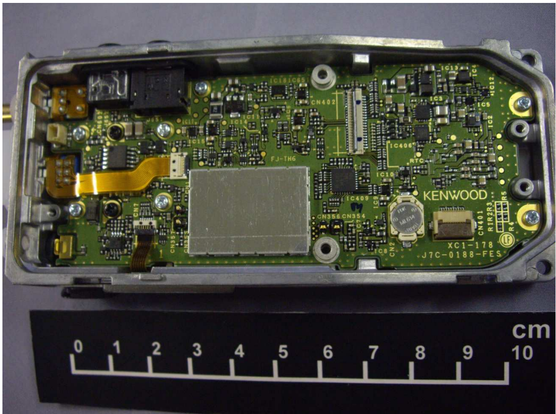
Top Internal View of TX-RX Unit
