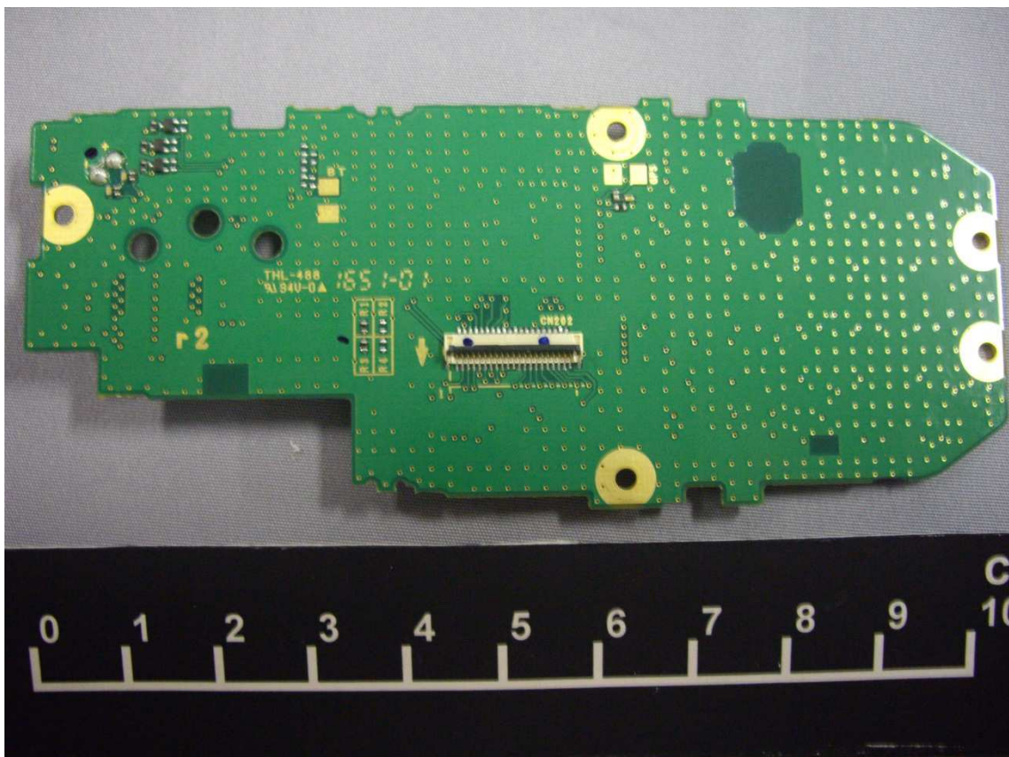
DISPLAY Unit of NX-3220-K2 (Bottom)
