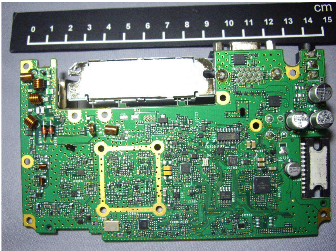
TX-RX unit (Bottom)
